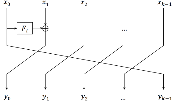
Fig. 1. Round i of Type-1 Feistel Scheme
