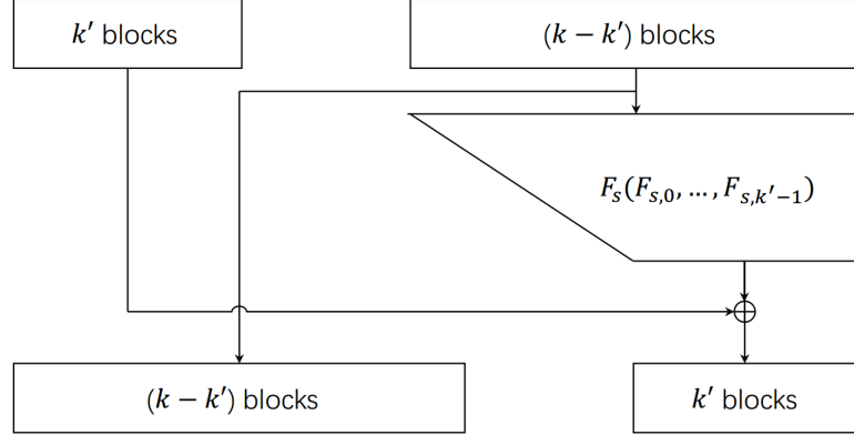
Fig. 4. Round s of Unbalanced Feistel Scheme
