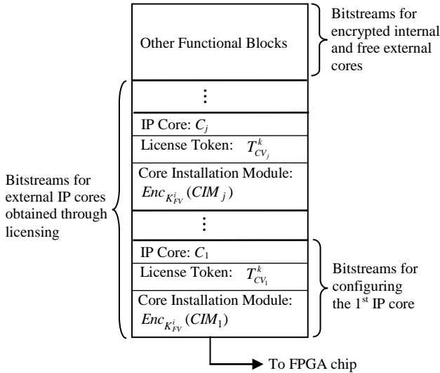
Fig. 4. Queue of design modules in external NVM of device k in batch i .
