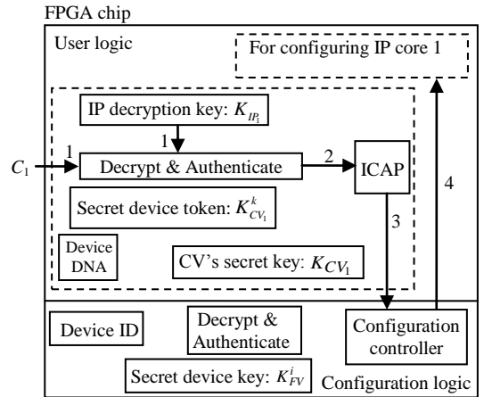
(c). Steps for configuring IP_1 with K_{IP_1}
