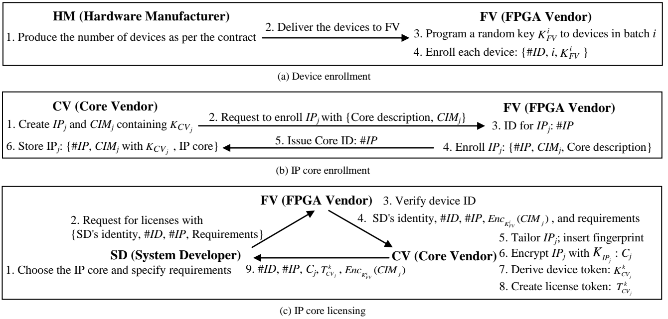
Fig. 3. Proposed protocol for the per-device IP licensing scheme.
