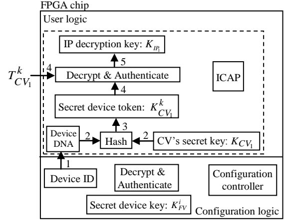
(b) Steps for establishing the secret IP key K_{IP_1}
