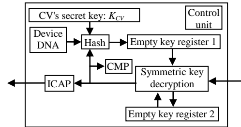
Fig. 2. Block diagram of the core installation module (CIM).
