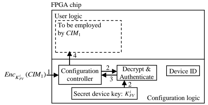
(a) Steps for implementing the encrypted CIM_1
