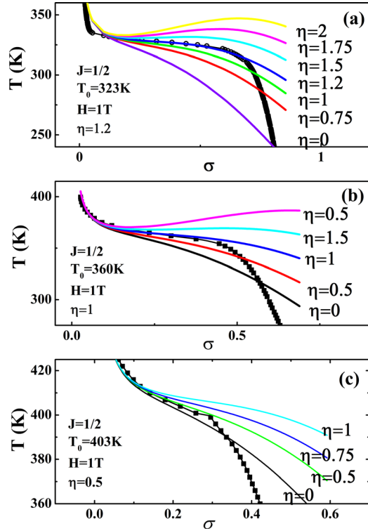
FIG. 2. Experimental temperature dependence of relative magnetization in 1 T external magnetic field of Ge0.26, Ge0.3, and Ge0.32 alloys (curves with symbol) compared to the modeling results of Bean-Rodbell Model for a range of \eta (plain curves).
