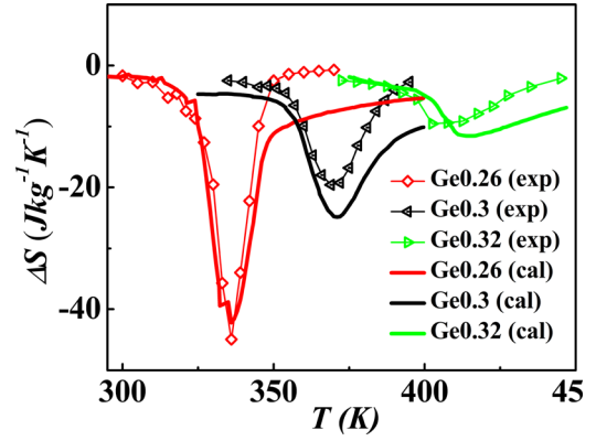
FIG. 3. Theoretical and experimental results of temperature dependence of isothermal magnetic entropy change for magnetic field change from 0 to 5 T in Ge0.26, Ge0.3, and Ge0.32 alloys.
