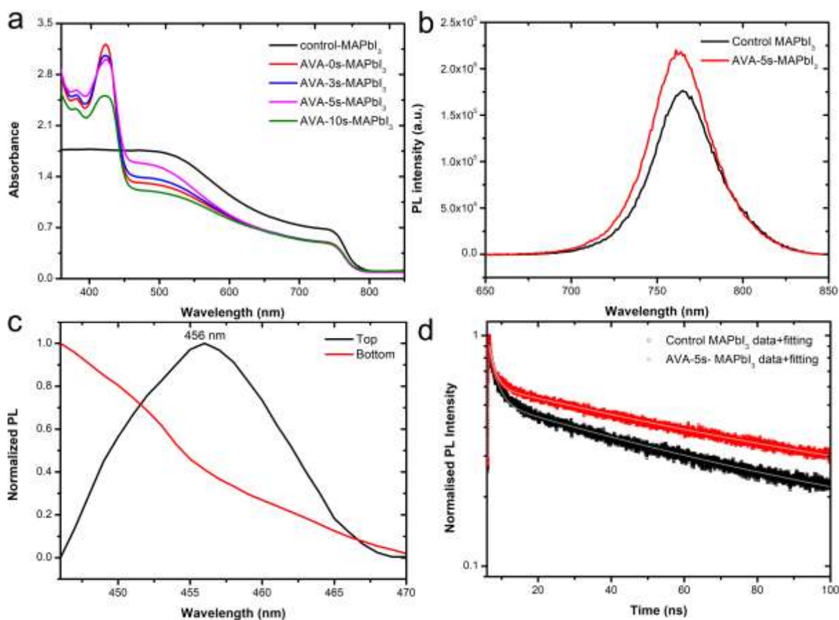
Figure 2. Optical characterization results of the perovskite samples. a) UV-vis optical absorption spectra of the control 3D perovskite films and 2D@3D perovskite films with different flash annealing duration (AVA-0s-MAPbI 3 , AVA-3s-MAPbI 3 , AVA-5s-MAPbI 3 , AVA-10s-MAPbI 3 ). b) PL spectra, excitation at 405 nm, of the control 3D perovskite and
