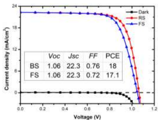
Figure S5. J-V results of the best solar cell (AVA-5s-MAPbI 3 ) measured under simulated AM 1.5 radiation and dark conditions with forward scan (FS) and reverse scan (RS).
