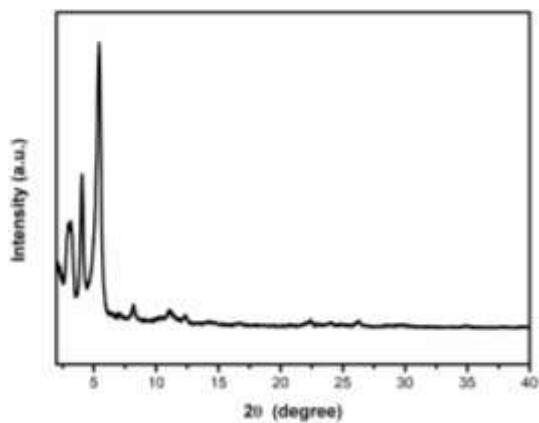
Figure S4. XRD results of 2D perovskite-(AVA) 2 PbI 4 .
