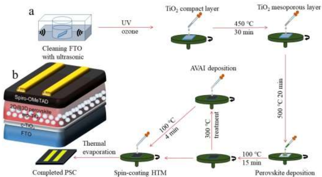
Figure S3. a) The schematic of the different PSCs fabrication processes and b) of the prepared 2D@3D PSC.
