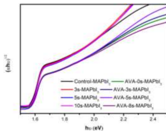
Figure S2. Corresponding Tauc plots of the various perovskite films.
