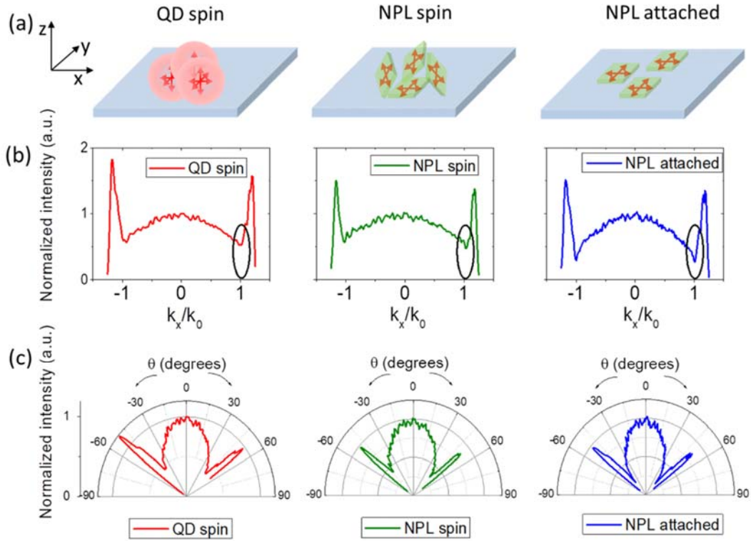
Figure 5. Angle and k -space dependent p-polarized emission characteristics of spin-coated spherical QDs, spin-coated NPLs, and attached NPLs. (a) A schematic representation of film of spin-coated QDs, spin-coated NPLs and NPLs via linker-based attachment on glass substrates. (b) k -dependent and (c) \theta -dependent intensity profile of p-polarized spectra of all samples. k_0 is the wavevector in air. Angle-dependent polar plots were obtained by performing Jacobian conversion on the k -space spectra. The substrate is on the x - y plane. The plane of incidence for the emitted light is on the x - z plane. The collected radiation emitted in the x - z plane (defined as p-polarized) emanates from a distribution of emitter dipoles oriented in-plane ( p_x ) and out-of-plane ( p_z ) of the substrate.
