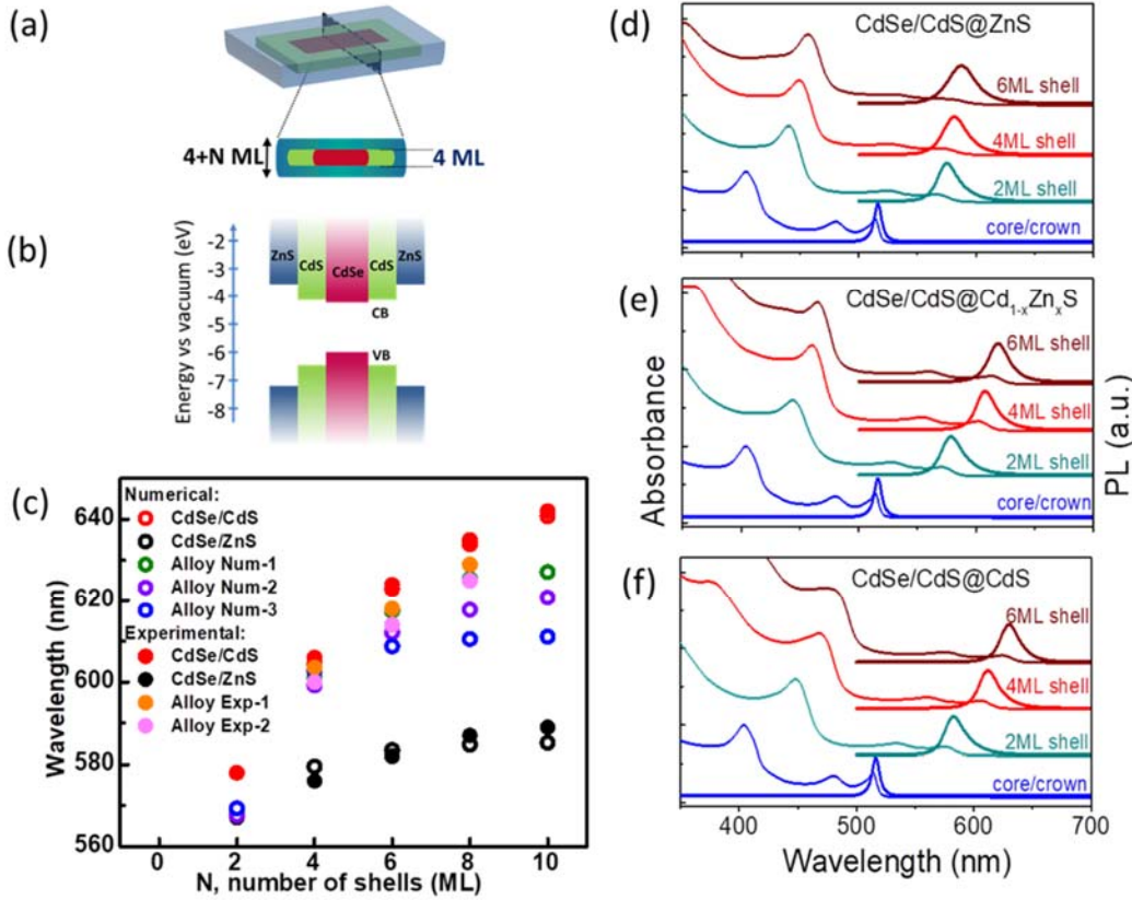
Figure 1. Emission and absorption characteristics of CdSe/CdS@Cd 1-x Zn x S core/crown@shell NPLs. (a) A schematic structure of the proposed core/crown@shell NPLs where N represents the number of shell layers on top of 4 ML core/crown seeds; (b) the energy band diagram showing relative positions of CdSe, CdS and ZnS bandgaps; and (c) calculated energies (open circle symbol) of the heavy hole transitions of CdSe/Cd 1-x Zn x S core/shell NPLs, by solving stationary Schrödinger equation considering the effective mass approximation. The different ‘x’ values in Cd 1-x Zn x S for N = 2, 4, 6, 8, 10 MLs of shell, respectively, in different alloy shell samples are: Alloy Num-1: (x = 0.10, 0.18, 0.33, 1.00, 1.00), Alloy Num-2: (x = 0.2, 0.4, 0.6, 0.8, 1.0), and Alloy Num-3: (x = 0, 1, 1, 1, 1). The solid circle symbols represent energy of the heavy hole transitions from experimental results. (d)-(f) The absorbance and PL spectra of NPLs with (d) Zn-only, (e) gradient alloy, and (f) Cd-only shells on top of CdSe/CdS core/crown NPLs.
