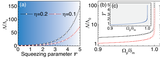
FIG. 3. The enhanced effective spin-spin coupling strength \Lambda varying with the squeezing parameter r \in [0, 5] (a) and the pump amplitude \Omega_p/\delta_m \in [0.9, 1) (b), with different constraint \eta = 0.2 and \eta = 0.1 . (c) The squeezing parameter r versus \Omega_p/\delta_m . Here we assume that the effective spin-spin coupling strength without the two-phonon drive ( r = 0 ) is \Lambda_0 \simeq 0.1\lambda .
