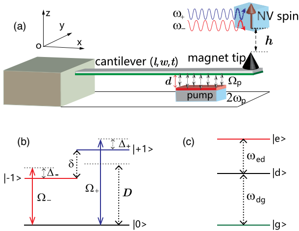
FIG. 1. (a) Schematic of a single NV center magnetically coupled to a silicon cantilever mechanical resonator, whose spring constant is periodically modulated. The NV center is set just on the top of the corresponding magnet tip with a distance h \sim 25 nm. (b) Level diagram of the driven NV center electronic ground states |m_s = 0, \pm 1\rangle . (c) Level diagram of the dressed spin basis states.
