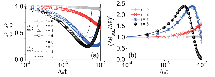
FIG. 4. (a) Metrological spin squeezing parameter \xi_R^2 and spin squeezing parameter \xi_S^2 , and (b) metrological gain (\Delta\theta_{\text{SQL}}/\Delta\theta)^2 versus time under different values for the mechanical amplification parameter r , with the initial state of the NV spins |g \cdots g\rangle and the coefficients \delta_{dg} = 0 , \Lambda_0 \simeq 0.1\lambda , \gamma_{\text{NV}} = 0.001\lambda , and N = 6 .
