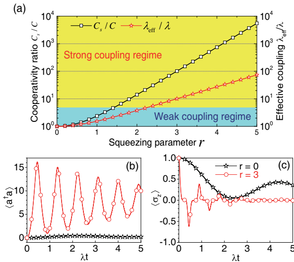
FIG. 2. (a) Cooperativity enhancement C_S/C and the spin-phonon coupling enhancement \lambda_{\text{eff}}/\lambda versus the squeezing parameter r , with \delta_m = 10\lambda . (b), (c) Quantum dynamics of the mechanical resonator and NV spin with the two-phonon drive ( r = 3 ) or without it ( r = 0 ), where the parameters are \delta_m = \lambda , \delta_{dg} = 0 , \Gamma_m^S = \gamma_{\text{NV}} = 0.1\lambda . The mechanical mode and NV center are initially prepared in the vacuum state |0\rangle_m and dressed state |d\rangle , respectively.
