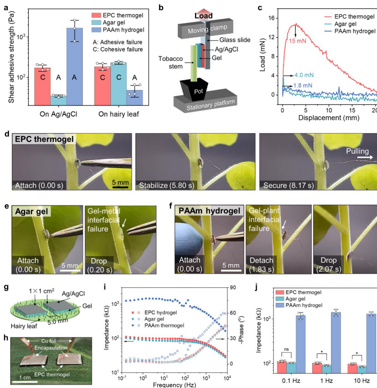
Figure 3. Adhesive and electrical properties of EPC thermogel. a , Histogram showing shear adhesive strengths of EPC thermogel, agar gel, and PAAm hydrogel on Ag/AgCl plates and hairy leaves of gloxinia (mean \pm s.d.). EPC thermogel fails cohesively regardless of substrates, implying robust interfacial adhesion. b , Schematic of the experimental setup for shear tests of gel-based electrodes on tobacco ( Nicotiana benthamiana ) stems. c , Representative load-displacement curves from the shear tests, showing substantially higher shear force of EPC thermogel-based electrodes than controls. Load is not converted to stress due to difficulty in accurately measuring contact area (roughly controlled at 1 cm 2 ). d-f , Snapshots of applying plate electrodes based on different hydrogels (electrode construction shown in Figure S12) on tobacco stems. Only did EPC thermogel secure the electrode firmly. g, h , Schematic ( g ) and photograph ( h ) showing the setup for measuring impedance of gel-based electrodes on hairy
