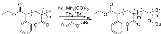
Scheme 3. Synthesis of block copolymers by the combination of RCMP and PROAD polymerizations
