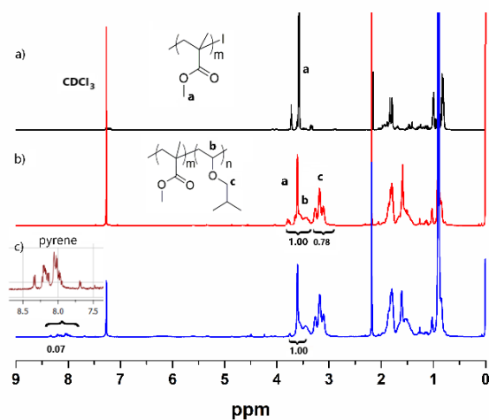
Figure 1. 1 H NMR spectra of a) PMMA, b) PMMA- b -PIBVE, c) pyrene functional PMMA- b -PIBVE.
