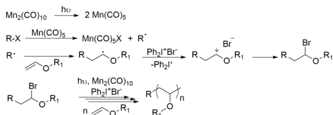
Scheme 2. Mechanism of PROAD polymerization of vinyl ethers.
