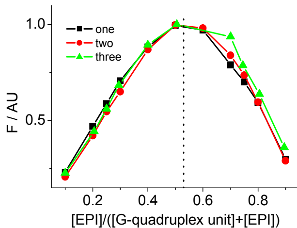
Figure S10. Job's plot analysis of the stoichiometric binding of EPI with DNAs of 5'-(TTA[Q]) n TTA-3' (n = 1, 2, 3) containing one, two, and three G-quadruplex units, respectively. Note that the values of X-axis are the G-quadruplex unit concentration.
