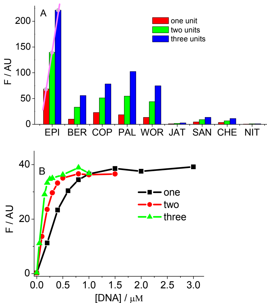
Figure S9. (A) Fluorescence intensity of the investigated isoquinoline alkaloids in the presence of DNAs (1 \mu\text{M} ) containing one, two, and three G-quadruplex units (5'-(TTA[Q] n )TTA-3' with n = 1, 2, 3 ), respectively. The concentrations of isoquinoline alkaloids are 1, 2, and 3 \mu\text{M} for the DNAs containing one, two, and three G-quadruplex units, respectively. The pink line shows the linear increase of EPI fluorescence upon increasing the number of G-quadruplex unit. EPI is the best alkaloid for targeting the long human telomeric G-quadruplexes. (B) Fluorescence titration of EPI (0.5 \mu\text{M} ) in 0.1 M \text{K}^+ by the addition of DNAs of 5'-(TTA[Q] n )TTA-3' ( n = 1, 2, 3 ) containing one, two, and three G-quadruplex units, respectively. Note that the values of X-axis are the DNA strand concentration. The results with the X-axis values based on the G-quadruplex unit concentration are given in the main text.
