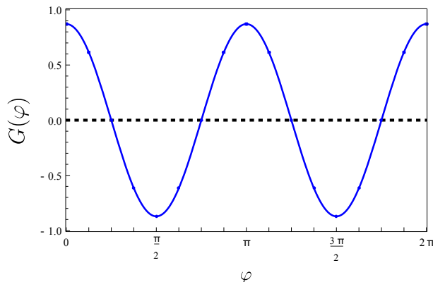
FIG. 1: Aspect's experiment and separability criterion: The solid line represents G(\varphi) defined in (7) measured by Aspect's experimental setup in 1981 [6]. The dashed line represents the prediction of a separable pure state in (2).
