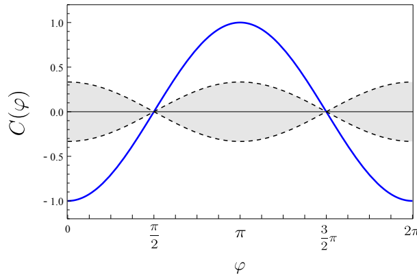
FIG. 2: Separable mixed state and Sakai's experiment: Shaded region is the prediction of the separable mixed quantum state in eq.(13), and the solid line is the experimental result C_{exp}(\varphi) = -\cos \varphi of Sakai et al. [7]
