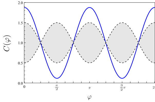
FIG. 3: Separable mixed state and Aspect's experiment in 1981 : Shaded region is the prediction of the separable mixed quantum state in eq.(23), and the solid line is the experimental result C_{exp}(\varphi) = 0.996 + 0.88 \cos 2\varphi of Aspect et al. [6].
