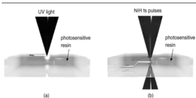
Figure 4. (a) UV light is absorbed at the surface of a photosensitive polymer thus leading structures only on the surface. (b) NIR light can be focused into the volume of the UV-sensitive resin and structures are only formed at the focal point. Picture taken from ref 42 with permission from Elsevier
