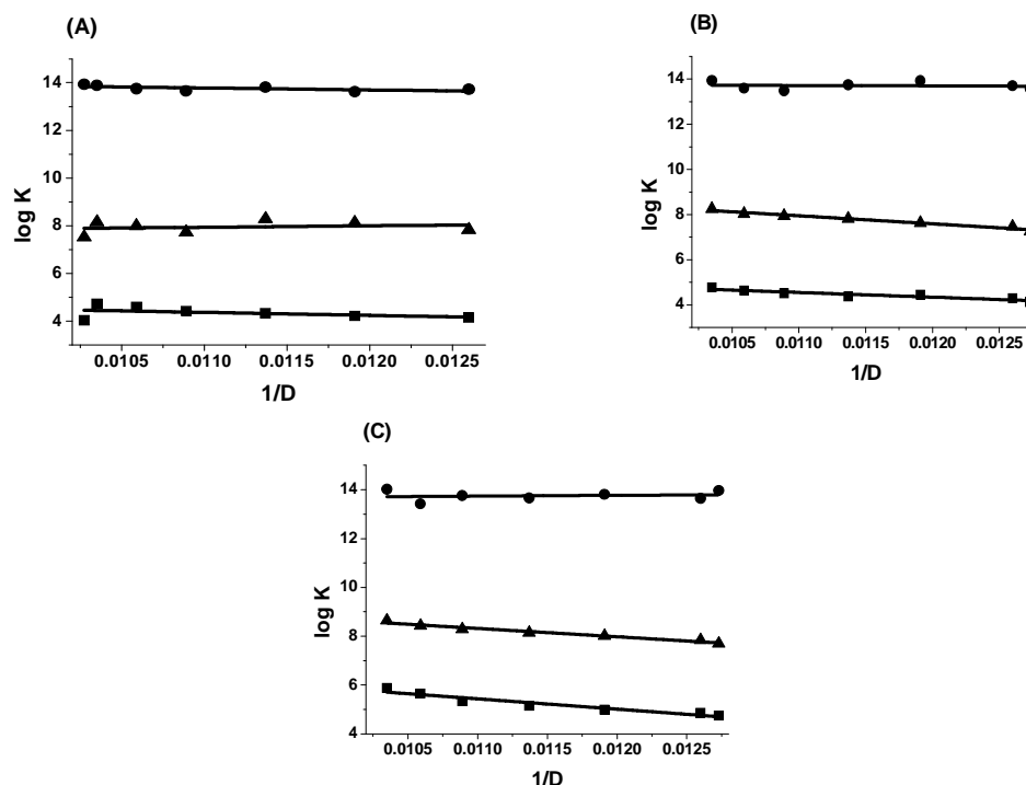
Figure 1. Variation of overall stability constant values of metal-5-SSA complexes with 1/D of Urea-water mixtures (a) Co(II); (b) Ni(II); (c) Cu(II); (■) log \beta_{ML} ; (▲) log \beta_{MLH} ; (●) log \beta_{ML_2} . Distribution Diagrams
