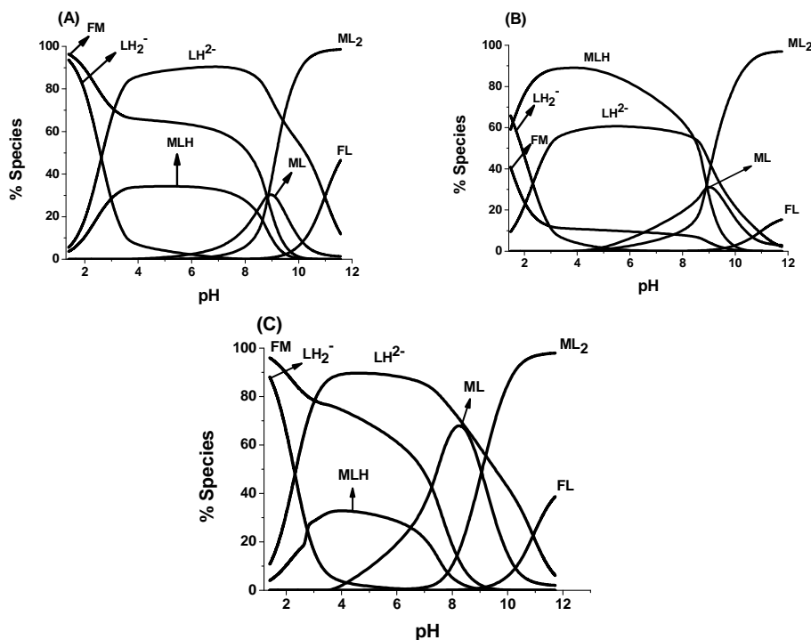
Figure 2: Distribution diagrams of binary complexes of 5-SSA in 5.8% w/v urea-water mixture: (a) Co(II), (b) Ni(II) and (c) Cu(II)
