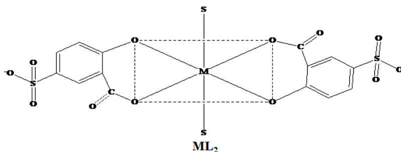
Figure 3: Structure of 5-SSA complexes, where S is either solvent or water molecules
