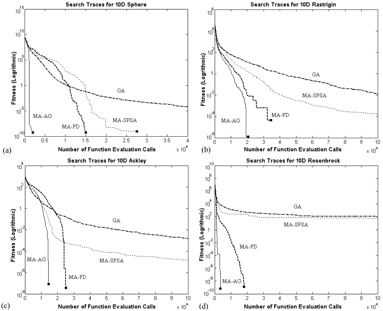
Fig. 2. Fitness versus number of function evaluation calls of test functions averaged over 25 runs.
