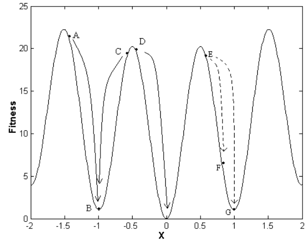
Fig. 3 Theoretical “traps” and effects of a fully/partially converged local search in one-dimensional Rastrigin
