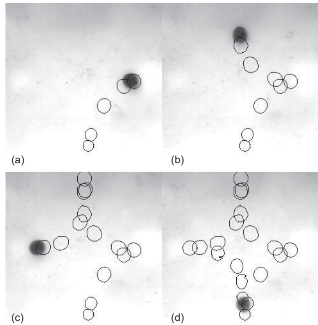
Figure 6. Ferrofluid droplet and its trajectory under two-dimensional actuation. The droplet is tracked every 2 seconds.
