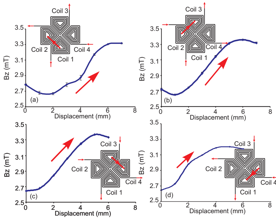
Figure 2. The measured magnetic flux normal to the coil plane and between the coil centers in the presence of permanent magnets. The uniform magnetic flux of approximately 3 mT in z direction contributed by the permanent magnets is included. The resultant field has only one peak between two adjacent coils on the actuation path. The ferrofluid droplet is attracted to this peak. The line connecting the coil centers shows the path along which the magnetic flux was measured: (a) Between coil 1 and coil 2; (b) Between coil 2 and coil 3; (c) Between coil 3 and coil 4; (d) Between coil 4 and coil 1.
