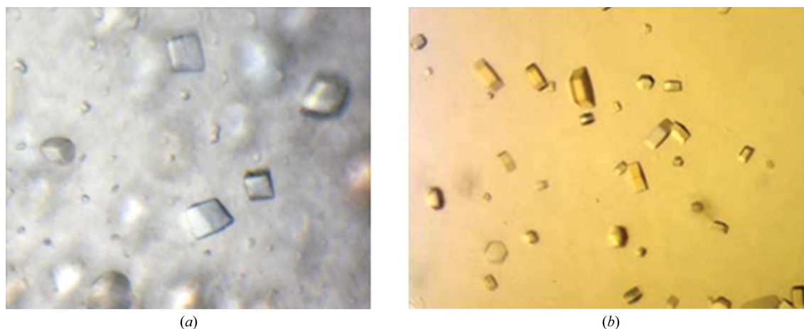
Figure 2 Crystals of the XccFimX^{EAL} -c-di-GMP and SeMet- XccFimX^{EAL} -c-di-GMP- XccPilZ_{1028} complexes. (a) XccFimX^{EAL} -c-di-GMP crystals grown in 0.2 M sodium formate pH 7.2, 20% PEG 3350 using the hanging-drop vapour-diffusion method at 277 K. These crystals reached average dimensions of 0.2 \times 0.2 \times 0.2 mm after one week. (b) SeMet- XccFimX^{EAL} -c-di-GMP- XccPilZ_{1028} crystals grown in 0.1 M HEPES pH 7.5, 0.2 M NaCl, 20% PEG 3K using the hanging-drop vapour-diffusion method at 277 K. These crystals reached average dimensions of 0.01 \times 0.01 \times 0.01 mm after three weeks.
