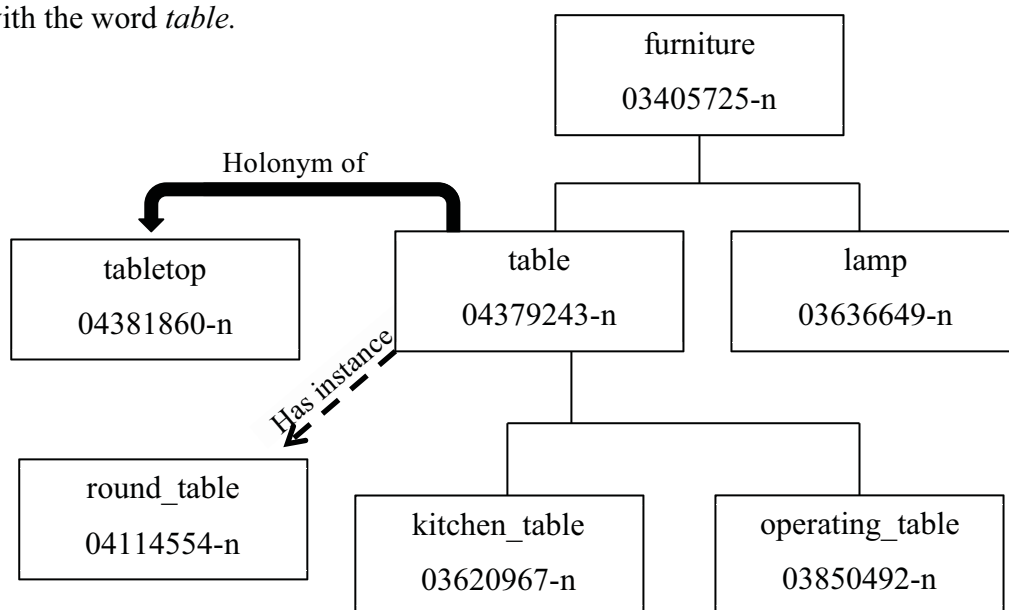
Figure 1. WordNet representation of table
