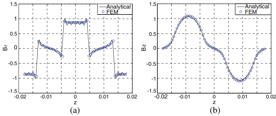
Figure 9. Field variation at the center of internal magnet area. (a) Variation of B_r . (b) Variation of B_z .
