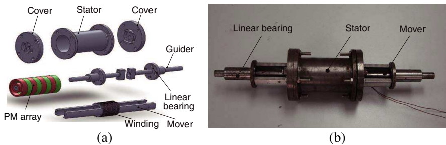
Figure 2. Linear machines with dual Halbach array. (a) 3D exploded view. (b) Research prototype.
