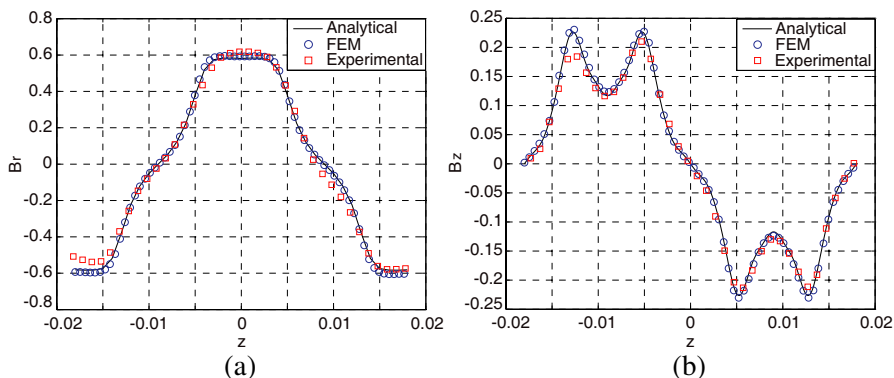
Figure 7. Magnetic field variation versus z at r = 12.5 mm. (a) B_r variation. (b) B_z variation.
