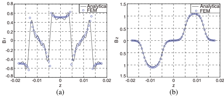
Figure 10. Field variation at the external magnet area. (a) Variation of B_r . (b) Variation of B_z .
