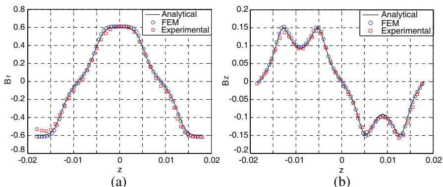
Figure 6. Magnetic field variation versus z at r = 12 mm. (a) B_r variation. (b) B_z variation.
