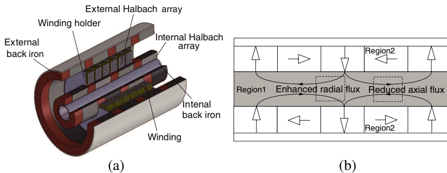
Figure 1. Tubular linear machine with dual Halbach array. (a) Schematic machine structure. (b) Magnetization and flux.
