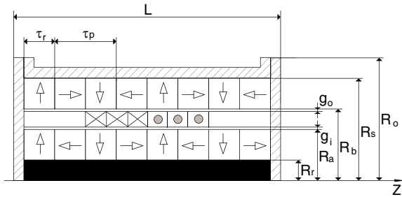
Figure 3. Structure of the research prototype.
