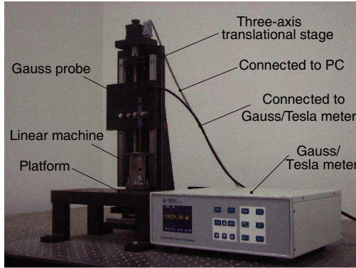
Figure 4. Experimental testbed for magnetic field measurement.
