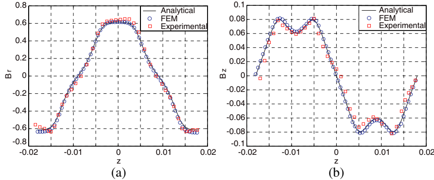
Figure 5. Magnetic field variation versus z at r = 11.5 mm. (a) B_r variation. (b) B_z variation.
