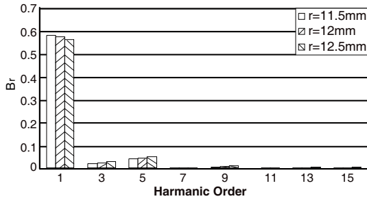
Figure 8. Harmonic content of radial flux density.
