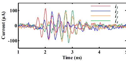
Figure 11. Simulated transient current at each tap for the four stages matched filter.
