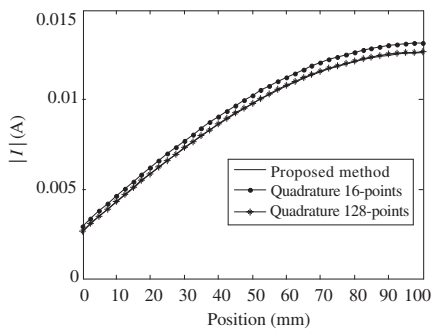
Figure 4. Current distributions of the short-circuited microstrip line at 350 MHz.
