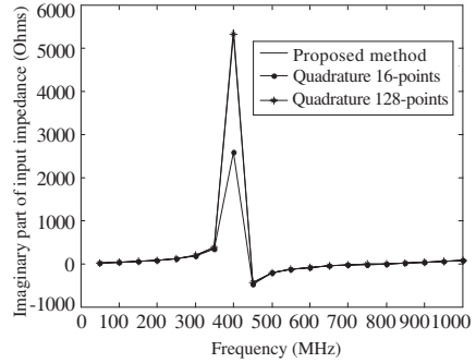
Figure 7. Input impedance of the short-circuited microstrip line (imaginary part).
