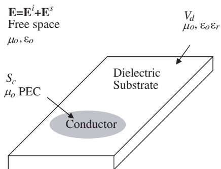
Figure 1. Finite-size printed circuit structure.
