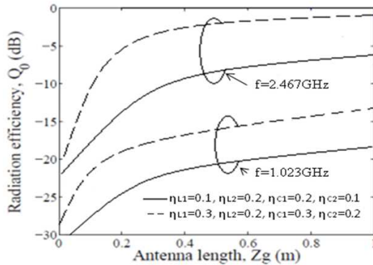
Figure 6. Radiation efficiency as a function of antenna length for different modulation indices.
