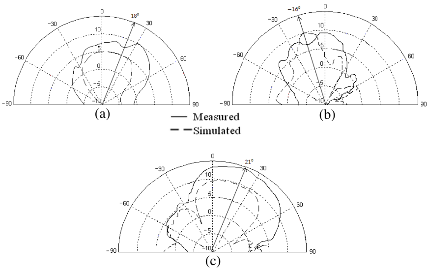
Figure 9. Measurement E -field radiation patterns in decibel scale at measured at (a) f_1 = 1.023 GHz, (b) f_2 = 2.467 GHz and (c) f_3 = 4.567 GHz.
