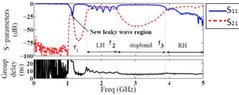
Figure 8. Measured frequency responses of TLs.
