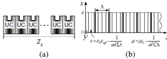
Figure 3. (a) Layout of the periodic TL. (b) Analytical model of double periodic dielectric on a ground plane.
