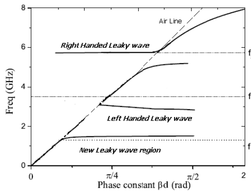
Figure 5. Dispersion characteristics of the double periodic TL based on singular perturbation procedure, quasi-static TM mode.
