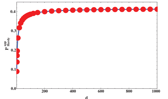
FIG. 1. (Color online) Plot of P_{\text{Hardy}}^{\text{app}} from d = 2 to 1000.
