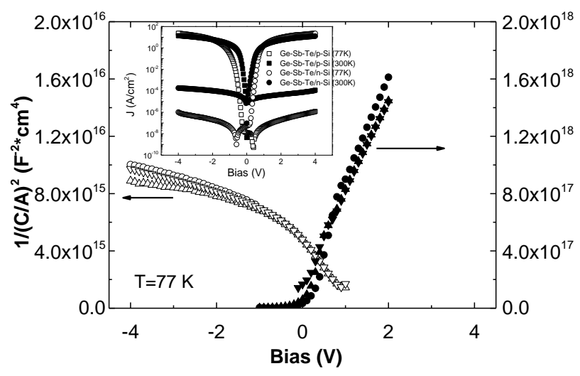
Figure 4. Mott-Schottky plots for unimplanted Ge-Sb-Te formed on n-type (open symbols) and p-type (filled symbols) silicon measured at frequencies of 100 kHz ( \circ, \bullet ), 200 kHz ( \blacktriangle, \triangle ), 400 kHz ( \blacktriangledown, \triangledown ), and 1 MHz ( \blacklozenge, \lozenge ) at 77K. The inset shows JV -curves taken at 300K (filled symbols) and 77K (open symbols).
