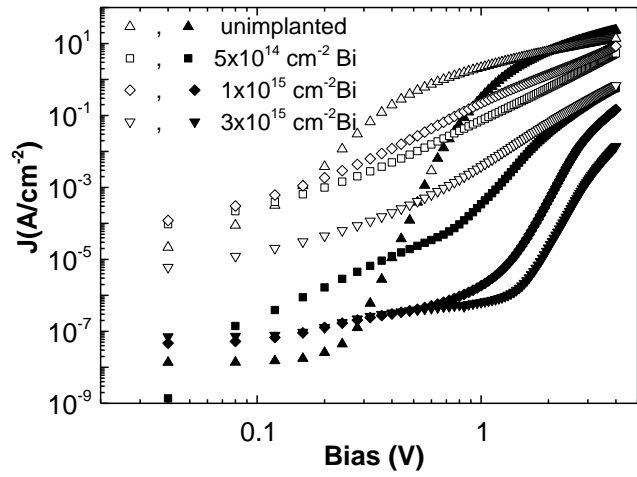
Figure 3. Forward current JV -characteristics for Ge-Sb-Te HJs formed on n-type silicon before implantation ( \blacktriangle, \triangle ) and subjected to different doses of the Bi implant: 5 \times 10^{14} \text{ cm}^{-2} ( \square, \blacksquare ), 1 \times 10^{15} \text{ cm}^{-2} ( \blacklozenge, \lozenge ), 3 \times 10^{15} \text{ cm}^{-2} ( \blacktriangledown, \triangledown ). Open symbol and filled symbols correspond to 300K and 77K, respectively.
