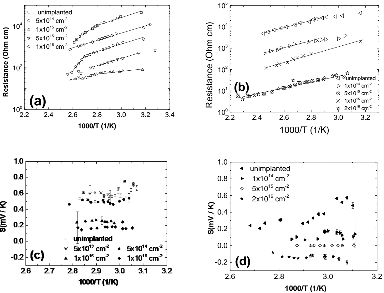
Figure 1. The resistivity \rho for Ge-Sb-Te and GeTe films is represented using open symbols on panel (a) and panel (b), respectively; the slope of the Seebeck coefficient S is shown by filled symbols on panel (c) and on panel (d) for Ge-Sb-Te and GeTe, respectively. Implantation doses of Bi are denoted as the following: 5 \times 10^{13} \text{ cm}^{-2} ( \ast ), 5 \times 10^{14} \text{ cm}^{-2} ( \bullet , \circ ), 1 \times 10^{15} \text{ cm}^{-2} ( \blacktriangle , \triangle ), 5 \times 10^{15} \text{ cm}^{-2} ( \blacktriangledown ), 1 \times 10^{16} \text{ cm}^{-2} ( \blacklozenge , \diamond ) for Ge-Sb-Te; 1 \times 10^{14} \text{ cm}^{-2} ( \blacktriangleright , \triangleright ), 1 \times 10^{15} \text{ cm}^{-2} ( \times ), 5 \times 10^{15} \text{ cm}^{-2} ( \otimes , \oplus ), 2 \times 10^{16} \text{ cm}^{-2} ( \star , \ast ) for GeTe. Squares ( \square , \blacksquare ) and left-turned triangles ( \triangleleft , \blacktriangleleft ) correspond to as-deposited Ge-Sb-Te and GeTe samples, respectively.
