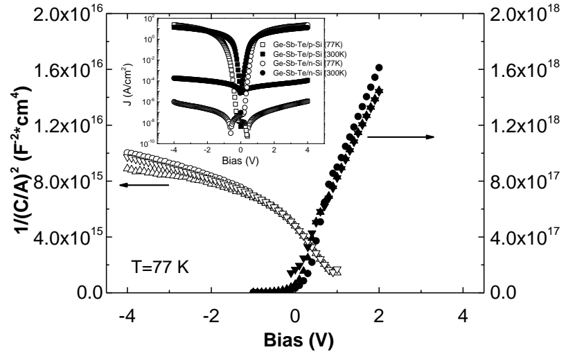
Figure 4. Mott-Schottky plots for unimplanted Ge-Sb-Te formed on n-type (open symbols) and p-type (filled symbols) silicon measured at frequencies of 100 kHz ( \circ, \bullet ), 200 kHz ( \blacktriangle, \triangle ), 400 kHz ( \blacktriangledown, \triangledown ), and 1 MHz ( \blacklozenge, \lozenge ) at 77K. The inset shows JV -curves taken at 300K (filled symbols) and 77K (open symbols).
