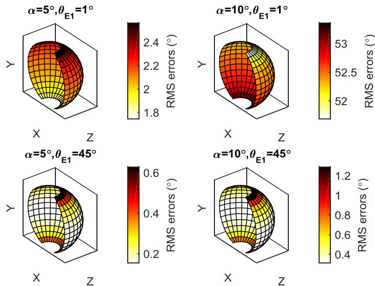
Fig. 5. Shoulder joint RMS errors of static poses (°)
