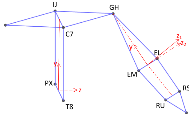
Fig. 1. Shoulder joint coordinate system determination alternatives
