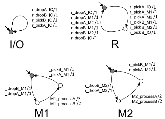
Fig. 2. Component Model
