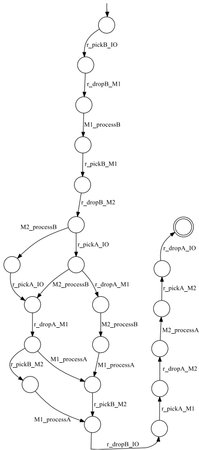
Fig. 4. Supremal Controllable Job Satisfaction Sublanguage
