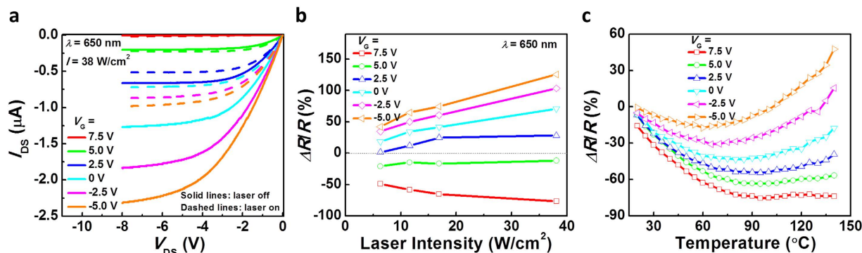
Figure 2. Photoresponse of the single chirality (9,8) nanotube transistor. (a) DC output characteristics ( I_{DS} - V_{DS} ) of a (9,8) nanotube transistor with a channel length of 100\ \mu\text{m} and a channel width of 200\ \mu\text{m} , measured before and after laser illumination ( \lambda = 650\ \text{nm} ). (b) Relative change in channel resistance as a function of laser intensity for various V_G . (c) Relative change in channel resistance as a function of sample temperature for various V_G .
