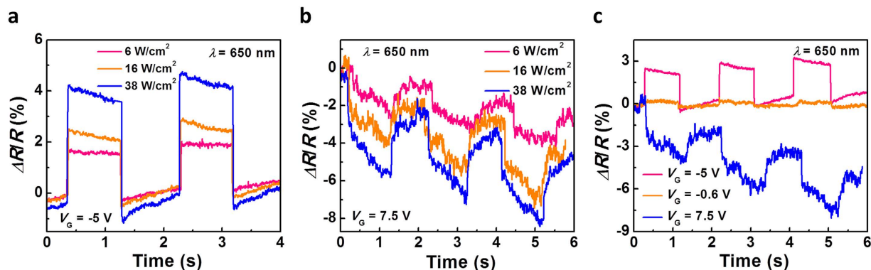
Figure 3. Photo-switching characteristics of the single chirality (9,8) nanotube transistor. (a) Time response of the photodetector under different laser intensities of 6, 16 and \sim 38 \text{W}/\text{cm}^2 measured at a V_G of -5 V. (b) Time response of the photodetector under different laser intensities of 6, 16 and 38 \text{W}/\text{cm}^2 measured at a V_G of 7.5 V. (c) Time response of the photodetector under a constant laser intensity of 16 \text{W}/\text{cm}^2 measured at various V_G values of -5 V, -0.6 V and 7.5 V.
