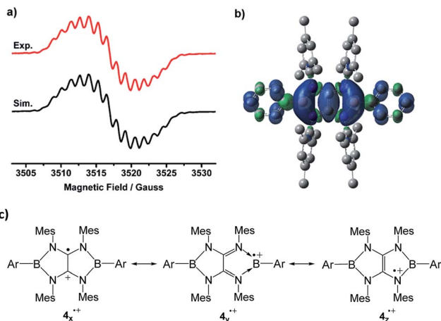
Fig. 4 (a) Experimental (red) and simulated (black) EPR spectra of 4a^{+\bullet} in fluorobenzene at room temperature. (b) The plot of the spin density of 4a^{+\bullet} . (c) The selected resonance forms of 4^{+\bullet} .
