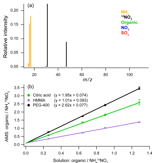
Figure 4. (a) Blank of the Kapton film using 1\text{ g L}^{-1} internal standard solution ( ^{15}\text{N} – ammonium nitrate). (b) Calibration curves made using an internal standard for solutions with three different organic compounds: citric acid, 4-hydroxy-3-methoxy-DL-mandelic acid (HMMA), and polyethylene glycol 400 (PEG-400). The error bars are \pm 1\sigma for five replicate injections.
