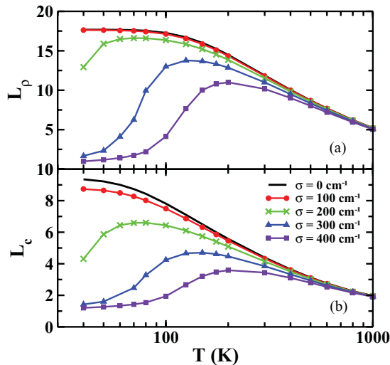
FIG. 10. (Color online) The coherence lengths (a) L_\rho and (b) L_c (b), calculated for LH2 as a function of temperature for increasing strength of the annealed disorder. The solid (black) line is obtained from the Boltzmann populations without any disorder. The widths of the annealed disorder distribution of 100, 200, 300, and 400 \text{cm}^{-1} are indicated by the (red) line with dots, (green) line with crosses, (blue) line with triangles, and (purple) line with squares, respectively.
