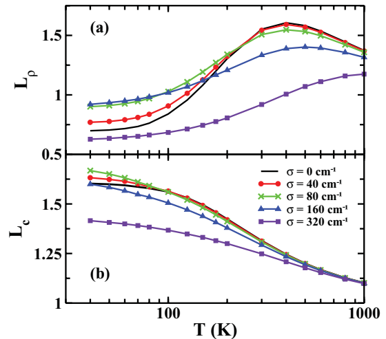
FIG. 11. (Color online) The coherence lengths (a) L_\rho and (b) L_c (b), calculated for FMO as a function of temperature for increasing static disorder. The solid (black) line is obtained from the Boltzmann populations without any static disorder. The widths of the static disorder distribution of 40, 80, 160, and 320 \text{cm}^{-1} are indicated by the (red) line with dots, (green) line with crosses, (blue) line with triangles, and (purple) line with squares, respectively.
