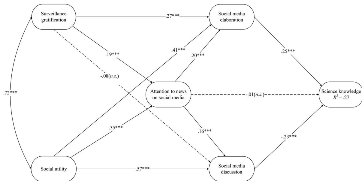
Figure 2. Structural equation model with standardized coefficients ( N = 901 ).
