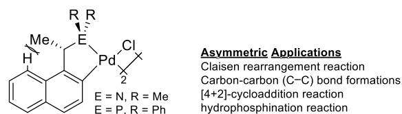
Figure 3. Chiral ( S )-1-naphthylethylamine cyclopalladated complex and its applications.
