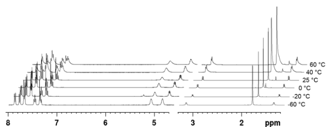
Figure 8. Variable temperature (VT) 1 H NMR studies on cycloiridated complex ( S C ,S N ,R Ir )-2 from -60 °C to 60 °C. The chemical shift range from 4.7 to 8.0 ppm has been magnified for clarity.
