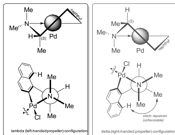
Figure 2. Possible conformations of cyclopalladated complex ( S )- N,N -dimethyl-1-naphthylethylamine.
