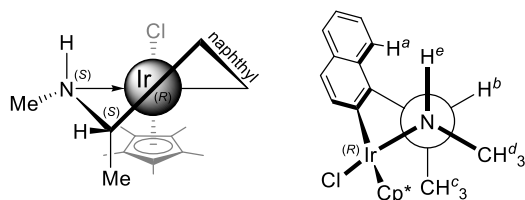
Figure 5. Preferred \lambda -conformation of cycloiridated complex ( S_C, S_N, R_{Ir} )-2.
