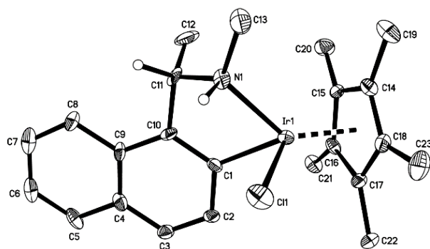
Figure 4. Molecular structure of cycloiridated complex ( S_C, S_N, R_{Ir} )-2 with thermal ellipsoids shown at 50% probability. Hydrogen atoms except H(C11) and H(N1) are omitted for clarity. Selected bond lengths and angles: N–Ir (2.151 Å), C–Ir (2.040 Å), Cl–Ir (2.425 Å), N–Ir–C (76.7°), N–Ir–Cl (82.5°), C–Ir–Cl (86.6°).
