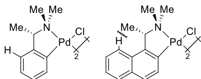
Figure 1. Chiral ( S )- N,N -dimethyl-1-phenylethylamine and ( S )- N,N -dimethyl-1-naphthylethylamine palladacycles.
