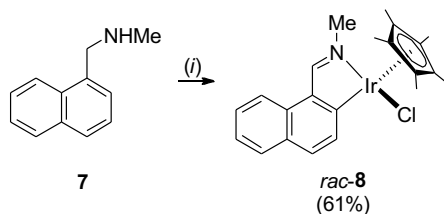
Scheme 3. Cycloiridation of N -methyl-1-naphthalene-methylamine 7 . Reaction conditions: (i) [\text{IrCp}^*\text{Cl}_2]_2 , NaOAc, 1,2-dichloroethane, 60 °C.
