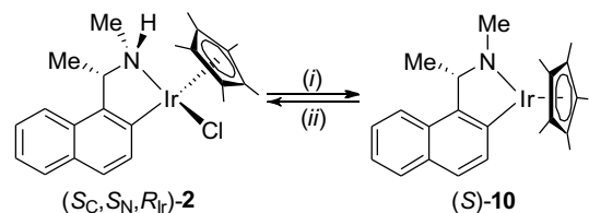
Scheme 4. Experiment on the stability of stereochemistry at nitrogen center. Reaction conditions: (i) KO t Bu, CD 2 Cl 2 ; (ii) HCl (aq.), room temperature.
