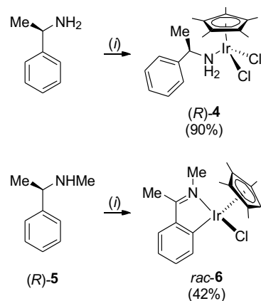
Scheme 2. Attempted direct cycloiridation of optically-active 1-phenylethylamine derivatives. Reaction conditions: (i) [IrCp^*Cl_2]_2 , NaOAc, CH_2Cl_2 , room temperature.
