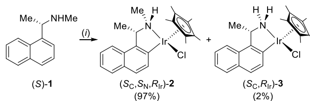
Scheme 1. Cycloiridation of optically-active secondary amine ( S )- 1 . Reaction conditions: (i) [IrCp^*Cl_2]_2 , NaOAc, CH_2Cl_2 , room temperature.
