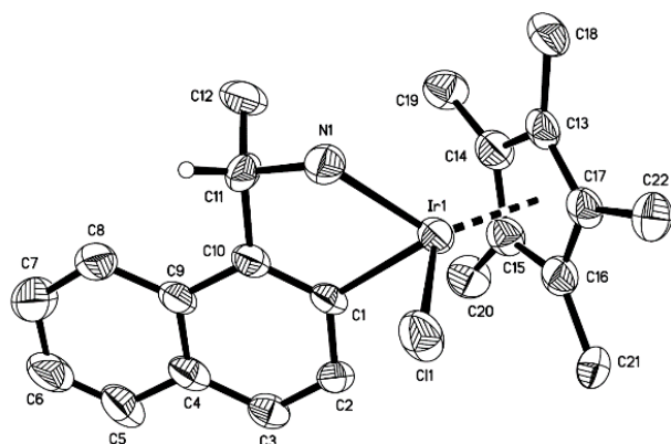
Figure 7. Molecular structure of cycloiridated complex ( S_C,R_{Ir} )-3 with thermal ellipsoids shown at 50% probability. Hydrogen atoms except H(C11) are omitted for clarity. Selected bond lengths and angles: N–Ir (2.122 Å), C–Ir (2.060 Å), Cl–Ir (2.431 Å), N–Ir–C (76.7°), N–Ir–Cl (82.5°), C–Ir–Cl (86.8°).
