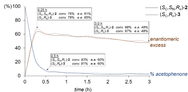
Figure 9. Conversion (blue) and enantiomeric excess (orange) profile of the asymmetric hydrogen transfer reaction of acetophenone by chiral cycloiridated complexes at -15\text{ }^{\circ}\text{C} .
