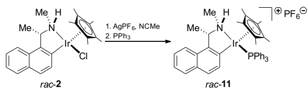
Scheme 5. Experiment on the stability of stereochemistry at iridium center during ligand exchange.
