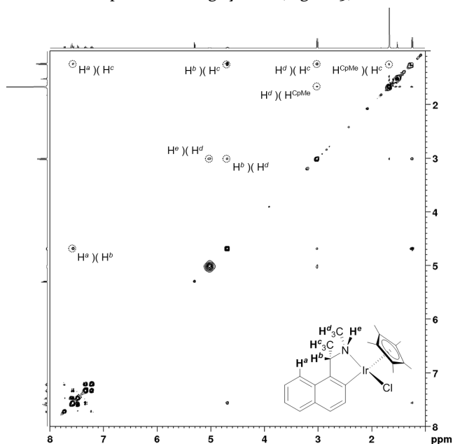
Figure 6. 2D ^1\text{H} - ^1\text{H} NOESY NMR spectrum of cycloiridated complex ( S_C, S_N, R_{Ir} )-2.
