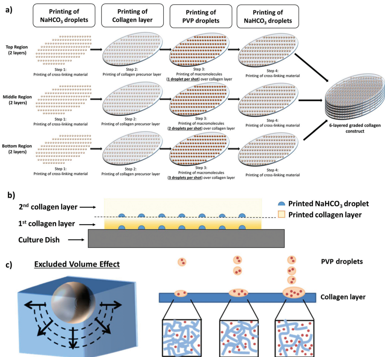
Fig. 4 (a) Schematic drawing of the Bioprinting-Macromolecular Crowding Process (BMCP); 6-layered hierarchical collagen constructs are printed by a bottom-up layer-by-layer fabrication approach. The microstructure within each printed collagen layer is manipulated by the number of printed PVP droplets at each pre-defined position as indicated by the red dots. (b) Schematic drawing depicting the collagen crosslinking with printed sodium bicarbonate ( \text{NaHCO}_3 ) droplets and bonding between the adjacent collagen layers. (c) Influence of PVP concentration on the collagen architecture; increasing the number of PVP droplets exert a more significant excluded volume effect (EVE) on surrounding collagen fibrils.
