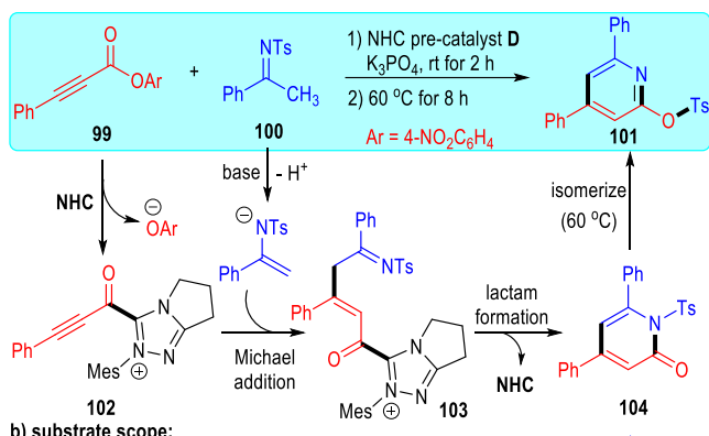
Scheme 14. NHC-catalyzed pyridine formation reaction with alkynyl carboxylic esters
