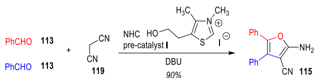
Scheme 17. NHC-catalyzed one-pot synthesis of 2-aminofuran with in situ formation of the acyldienemalononitrile substrate
