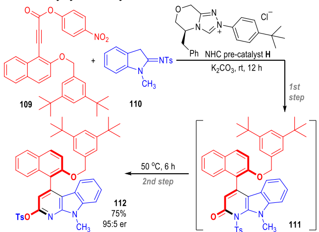
Scheme 15. NHC-catalyzed atropenantioselective reaction of alkynyl carboxylic ester and 2-sulfonamidoindoline
