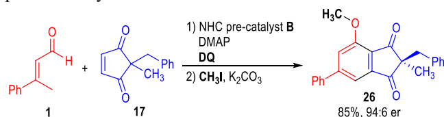
Scheme 4. NHC-catalyzed one-pot benzene formation / phenol methylation reaction
