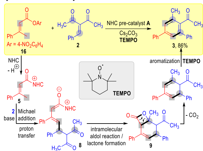
Scheme 2. NHC-catalyzed benzene formation via [3 + 3] cyclization of carboxylic ester and enone substrates
