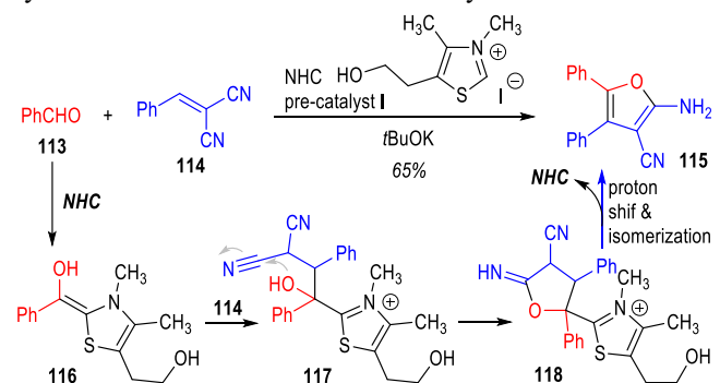
Scheme 16. NHC-catalyzed cascade Stetter- \gamma -ketonitrile cyclization reaction for 2-aminofuran synthesis
