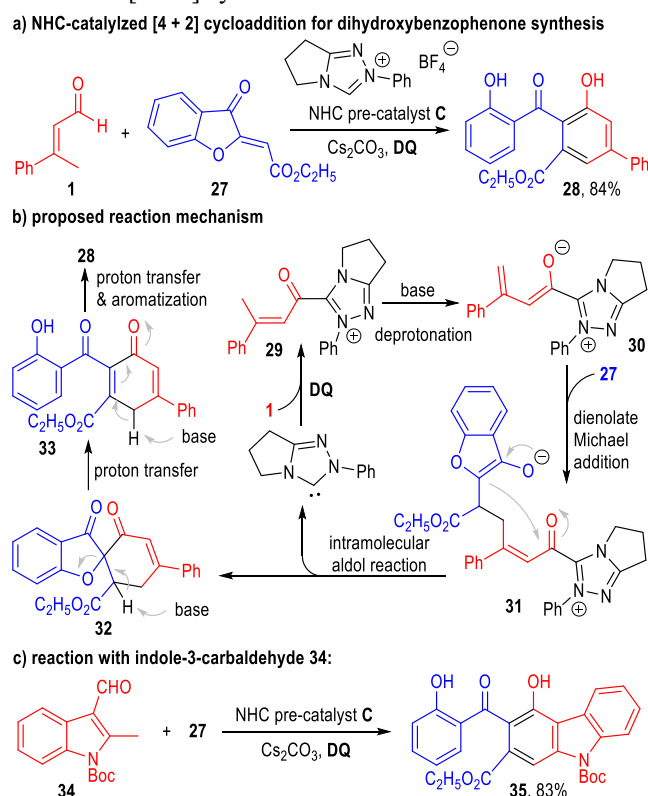
Scheme 5. NHC-catalyzed dihydroxybenzophenone formation via [4 + 2] cycloaddition reactions
