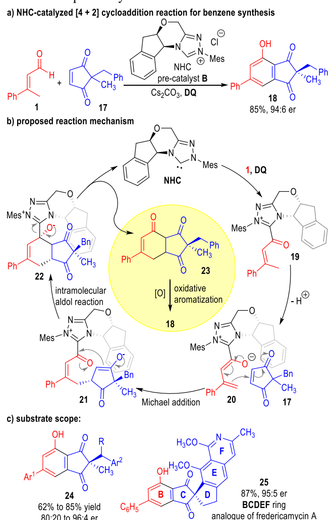
Scheme 3. NHC-catalyzed desymmetrization [4 + 2] cyclization for phenol synthesis
