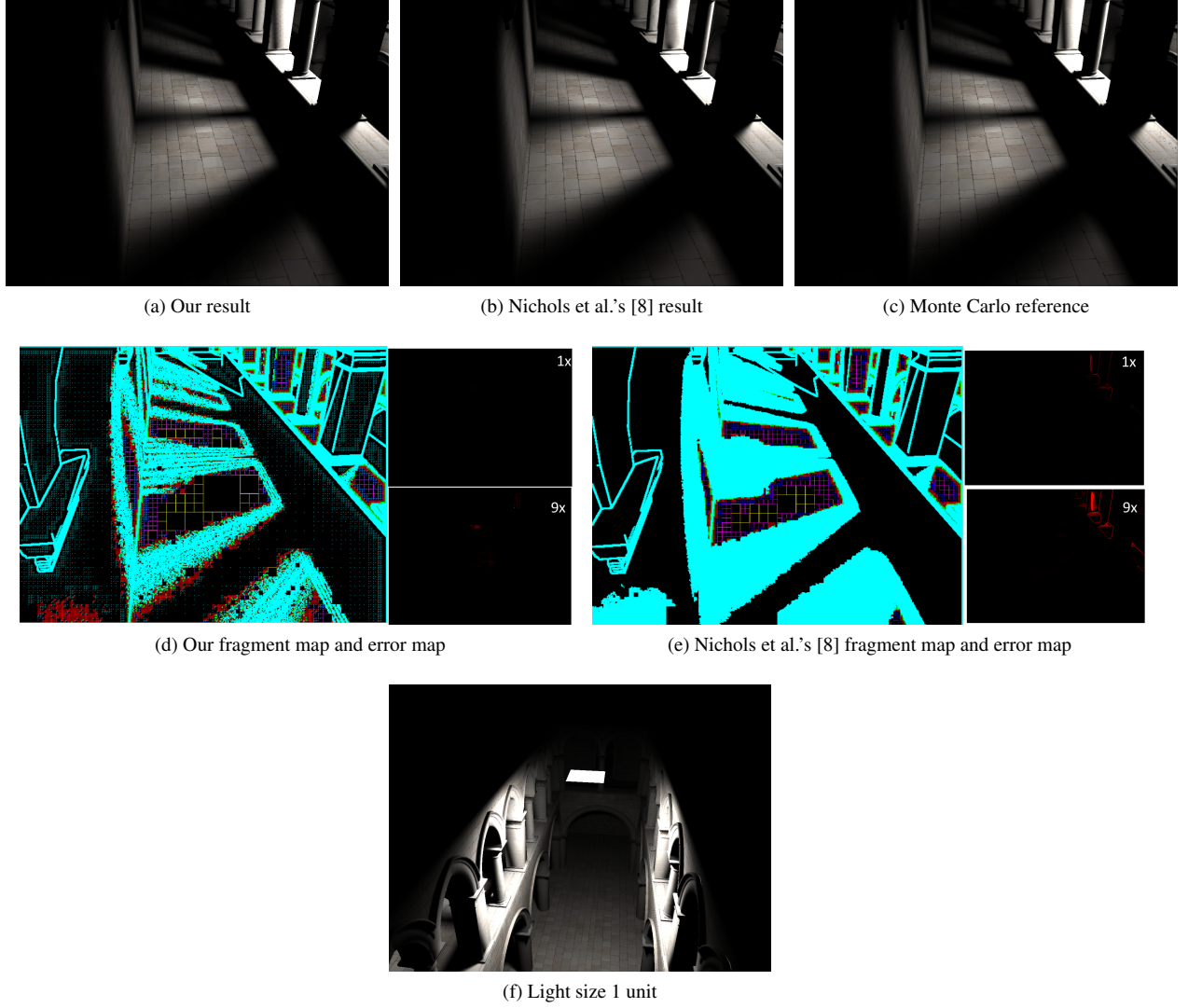
Figure 12: Rendering of the Sponza (McGuire Graphics Data) in 1280x960 pixels with direct illumination. In Figure 12d (right), we show the L2 error map in irradiance values (with scaling factor of 1x and 9x) between Figures 12a and 12c. The error map is mapped to the red color channel. Similarly Figure 12e (right) shows the L2 error map between Figures 12b and the reference image 12c. (f) shows the location and size of our planar light source.
