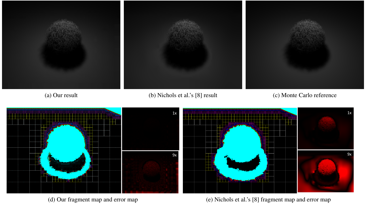
Figure 14: Rendering of the hairball object (McGuire Graphics Data) in 1280x960 pixels with direct illumination. In Figure 14d (right), we show the L2 error map in irradiance values (with scaling factor of 1x and 9x) between Figures 14a and 14c. The error map is mapped to the red color channel. Similarly Figure 14e (right) shows the L2 error map between Figures 14b and the reference image 14c.
