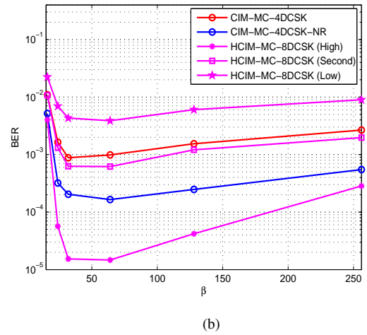
Fig. 11. BER performance of the CIM-MC- M -DCSK system, its noise-reduction scheme and its hierarchical-modulation scheme with different value of \beta (a) over AWGN at a bit SNR of 5 dB and (b) over multipath Rayleigh fading channel at a bit SNR of 20 dB.
