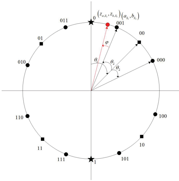
Fig. 2. A generalized 8-DCSK constellation.
