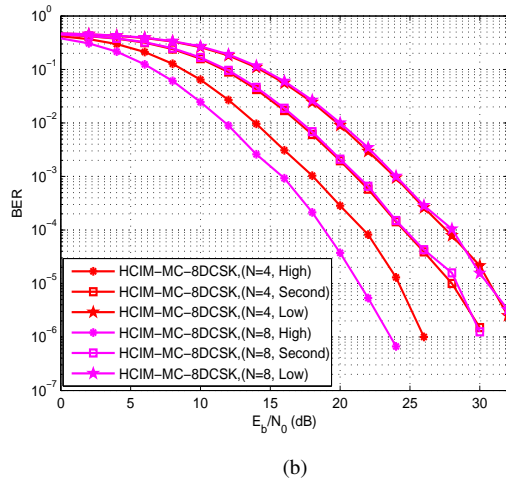
Fig. 9. BER performance of (a) the CIM-MC- M -DCSK system and its noise-reduction counterpart and (b) its hierarchical-modulation CIM-MC- M -DCSK system with different values of N over a multipath Rayleigh fading channel.
