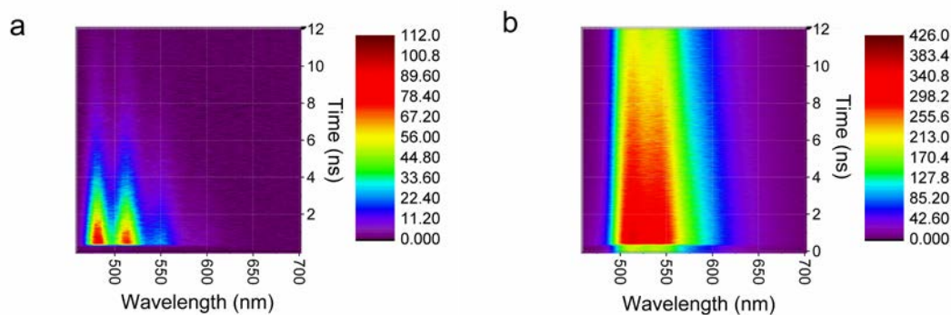
Figure 5. Fluorescence map of tetracene (a) and 5-azatetracene (b) in dichloromethane solution, \lambda_{\text{ex}} = 380 nm.
