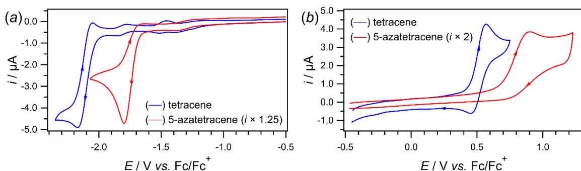
Figure 8. Comparison of (a) first reduction and (b) first oxidation process of 1 mM 5-azatetracene and tetracene. Cyclic voltammograms were recorded in DCM containing 0.1 M n\text{Bu}_4\text{NPF}_6 at a scan rate of 0.1 \text{ V s}^{-1} and using a 1 mm diameter GC working electrode at 298 \pm 2 \text{ K} in a Faraday cage.
