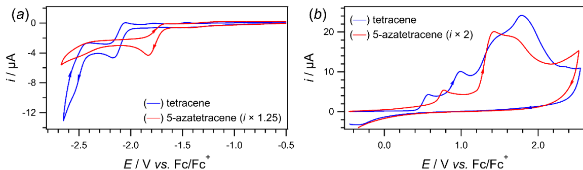
Figure 7. Cyclic voltammograms obtained in DCM containing 0.1 M n\text{Bu}_4\text{NPF}_6 at a scan rate of 0.1 \text{ V s}^{-1} and using a 1 mm diameter GC working electrode at 298 \pm 2 \text{ K} in a Faraday cage. (a) Reduction processes of 1 mM 5-azatetracene and tetracene. (b) Oxidation processes of 1 mM 5-azatetracene and tetracene
