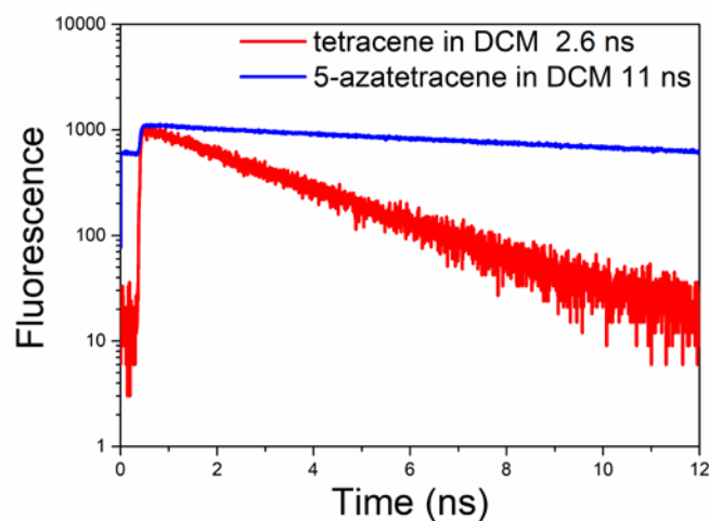
Figure 4. Fluorescence decay kinetics at 500 nm of tetracene and 5-azatetracene in dichloromethane solution, \lambda_{\text{ex}} = 380 nm.
