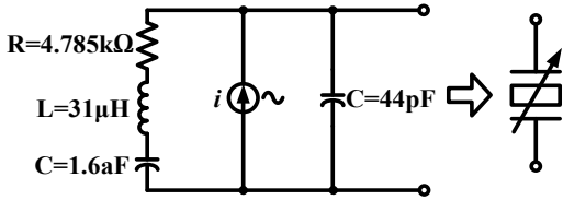
Figure 2. Equivalent simulation model for CMUT.
