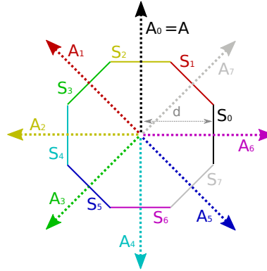
(b) Generation of an octagonal footprint.
