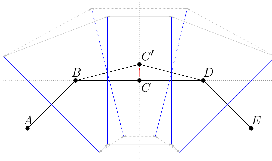
Figure 7.11.: A spring element with five points, four segments, eight normal rods and six springs connecting the end points of the rods. The position of the center point is spring-optimized along the perpendicular bisector of the line segment connecting its neighbours.
