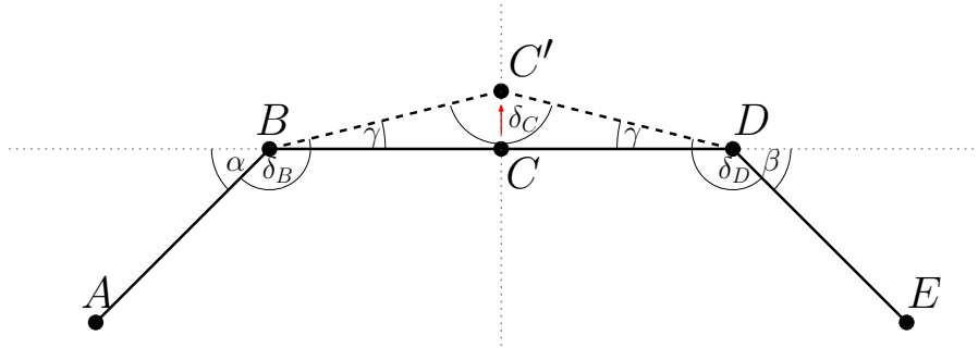
Figure 7.2.: Optimization of point C . Angles \alpha and \beta are given by the position of the points with respect to the dotted line g through B and D . C' is positioned on the perpendicular bisector of B and D such that \delta_C is the arithmetic mean of \delta_B and \delta_D . \gamma is used for the calculation.
