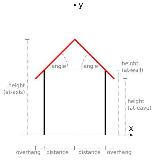
(a) Side parameters defined relative to one axis.
