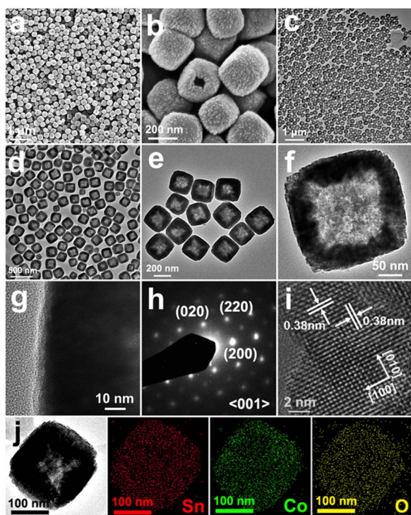
Figure 4 | Morphology and composition characterization. (a, b) FESEM images and (c–e) TEM images of CoSn(OH) 6 nanoboxes; (f) a nanobox with well-developed interior; (g) a TEM image showing the shell structure of a nanobox, on which a very thin layer of Co (III) species is covered on the outer surface; (h) SAED pattern of a single nanobox; (i) HRTEM image along a zone axis of \langle 001 \rangle ; (j) elemental mapping showing the homogenous dispersion of Sn, Co and O element in CoSn(OH) 6 nanoboxes.
