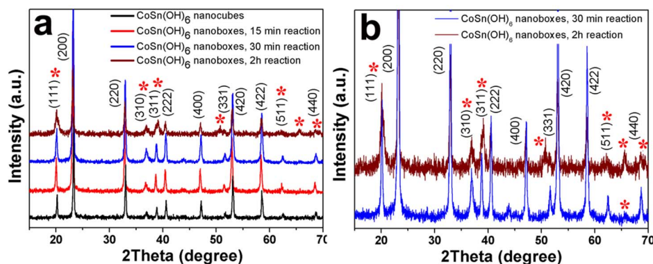
Figure 3 | Phase analysis. (a) XRD profiles of CoSn(OH) 6 nanocubes and nanoboxes obtained after the reaction of 15 min–2 h; (b) Enlarged XRD pattern of CoSn(OH) 6 sample obtained after 30 min and 2 h reaction, in which the signals of CoO(OH) phase are marked with red asterisks.
