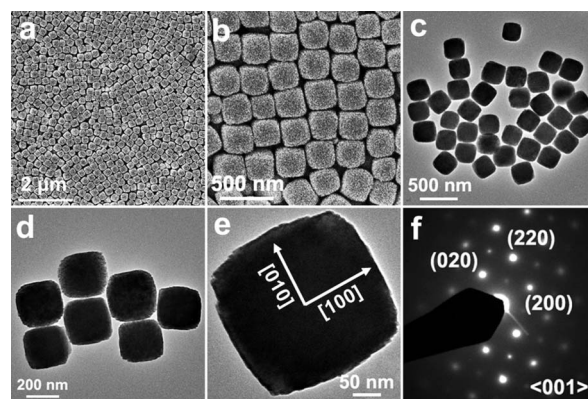
Figure 2 | Morphology characterization. (a, b) FESEM images and (c, d) TEM images of \text{CoSn}(\text{OH})_6 nanocubes. (e) a free-standing nanocube enclosed by six nominal {100} facets, and its corresponding SAED pattern (f) showing the perfect single-crystalline feature.
