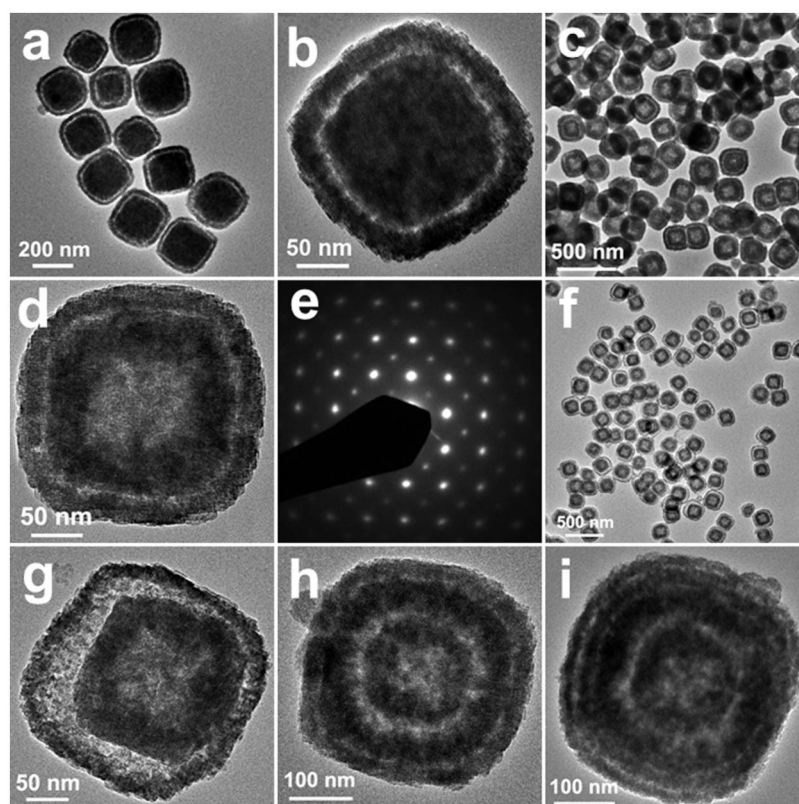
Figure 6 | Morphology characterization. TEM images of \text{CoSn}(\text{OH})_6 hollow architectures with multilevel interiors: (a, b) yolk-shell particles; (c, d) double-shelled nanoboxes; (e) SAED pattern of a double-shelled nanobox; (f, g) double-shelled nanoboxes with larger intershell cavities; (h) a triple-shelled nanobox; (i) a quadruple-shelled nanobox.
