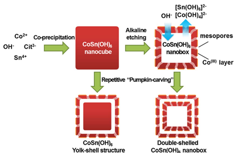
Figure 1 | Formation mechanism of \text{CoSn}(\text{OH})_6 hollow nanostructures. Schematic illustration for the formation of single-crystal \text{CoSn}(\text{OH})_6 yolk-shell particles and multishelled nanoboxes (citrate anion is denoted as \text{Cit}^{3-} ).
