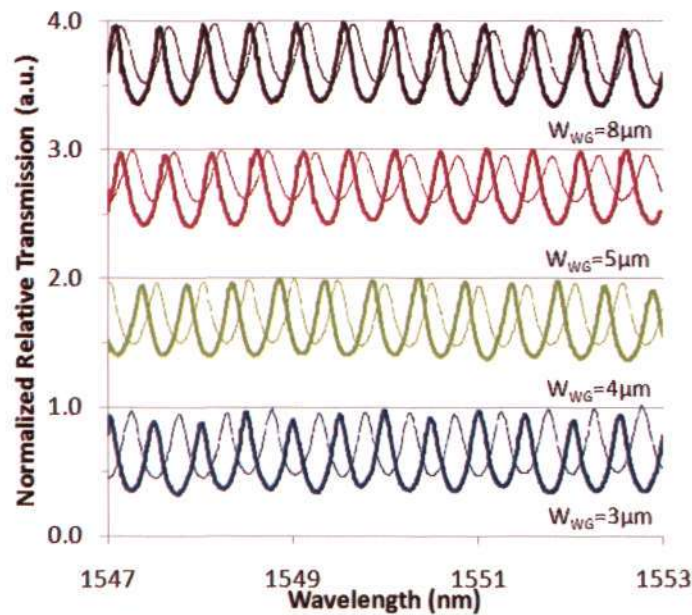
Fig. 3.4.3. Normalized transmission power for the FP resonance with waveguide widths of 3, 4, 5 and 8\mu\text{m} and length, L=0.66\text{mm} , as a function of wavelength. The bold lines are for TE polarization and the thin detached lines are for TM polarization
