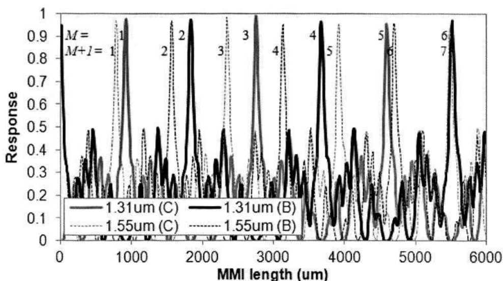
Fig.4.1.7. Simulations results of the periodicity of normalized TE mode power output response for a 23 \mu\text{m} wide Type II MMI wavelength filter versus MMI device length, L in \mu\text{m} .
