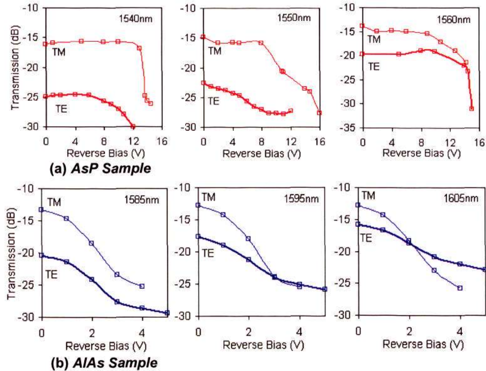
Fig.6.3.10. Transmission vs. reverse bias voltage measured for the (a) AsP Sample at the wavelengths 1540, 1550 and 1560nm and for the (b) AIAs Sample at the wavelengths 1585, 1595 and 1605nm for both polarizations
