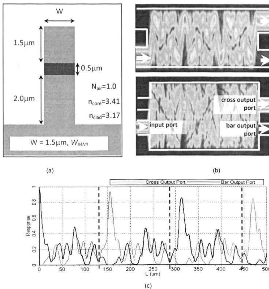
Fig.4.1.1. (a) Refractive indices and cross-section of the MMI devices and AWs; (b) Field distribution of a 2 \times 2 Type I (top) and Type II (bottom) MMI device where W_{\text{MMI}}=4.0\mu\text{m} and 7.7\mu\text{m} respectively. The access waveguides are 1.5\mu\text{m} wide with 1\mu\text{m} gap in between them. (c) Response vs. Length for a 2 \times 2 Type II MMI device. The dotted lines mark the positions of the output for MMI splitters that are designed as 3-dB couplers.
