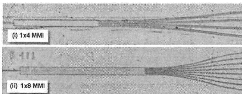
Fig. 3.5.5 (i) and (ii) are the microscope captures of the 1 \times 4 and 1 \times 8 MMIs fabricated for this experimental purpose
