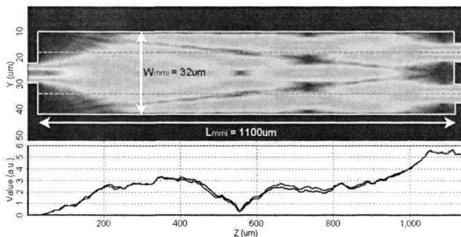
Fig. 6.3.6. 2D-BPM simulation of a 1x2 MMI device. The top half shows the field distribution of light in the device while the bottom part shows the output amplitude from both arms at different lengths of the device.
