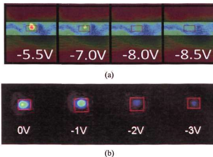
Fig.6.3.11. Bias voltage effect viewed from the Coherent MicronViewer Vidicon Camera Model 7290A for (a) AsP and (b) AlAs Sample
