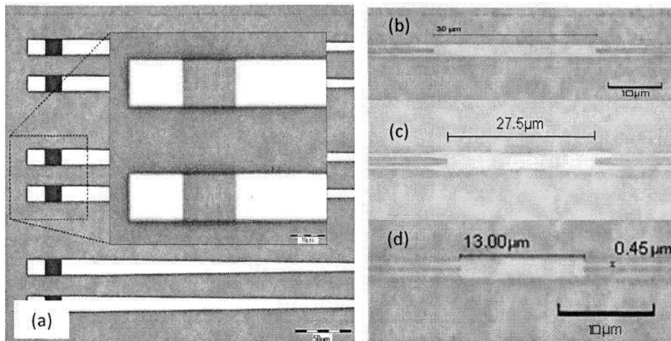
Fig.4.2.8. (a) Fabricated grating; (b) Type I MMIC with tapered AW; (c) Tapered MMIC and AW (d) Un-tapered MMIC
