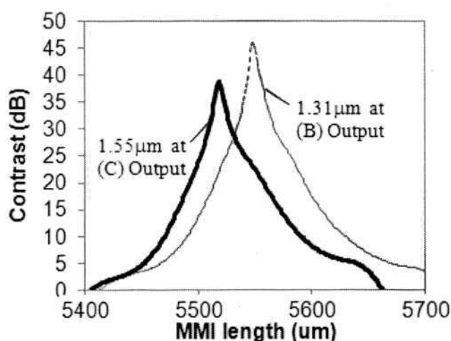
Fig.4.1.8. Contrast at opposing output arms as noted in the graph for the wavelength splitter design vs. MMI length around the designed length at the designed MMI length of L=5534\mu\text{m}
