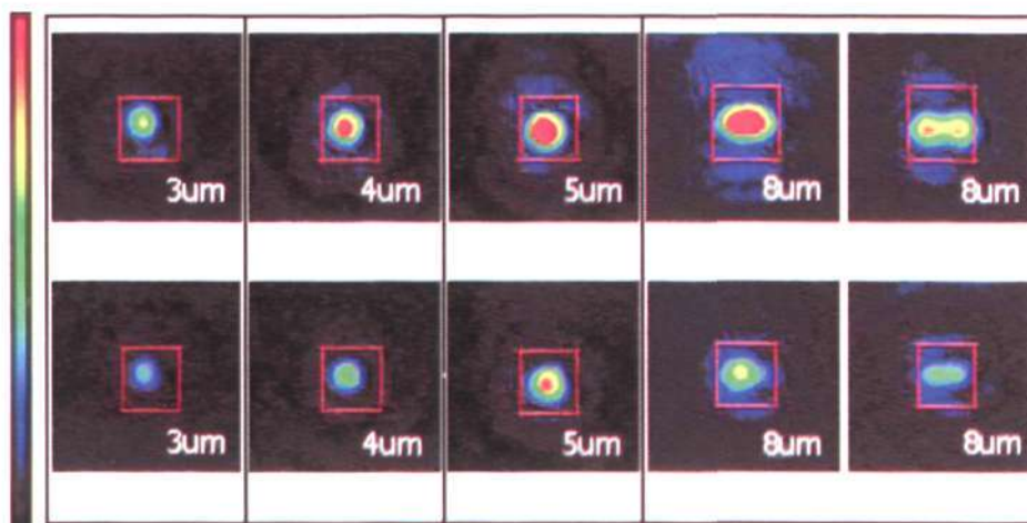
Fig.3.4.2. Images of modes captured using the vidicon camera. Top row shows captures of modes at brighter resonance and lower row shows captures of modes at dimmer resonance. For 8\mu\text{m} , higher order modes were easily excited and captured.
