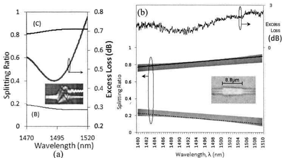
Fig.4.2.14. (a) Simulation and (b) experimental results for an 8.8\mu\text{m} long 80:20 (Cross: Bar) MMI splitter. For (a), the bold (C) and thin (B) lines represent the cross and bar results simulated for the device along with the simulated excess loss in dB. For (b), the bold and detached lines represent the cross and bar result line fit result obtained from the 8.8\mu\text{m} long device. Shaded area denotes measured shift in ratio when MMI length is varied from 8.4 to 9.2\mu\text{m} . Excess loss is plotted above the splitting ratio. Inset picture is a microscope capture of the device.
