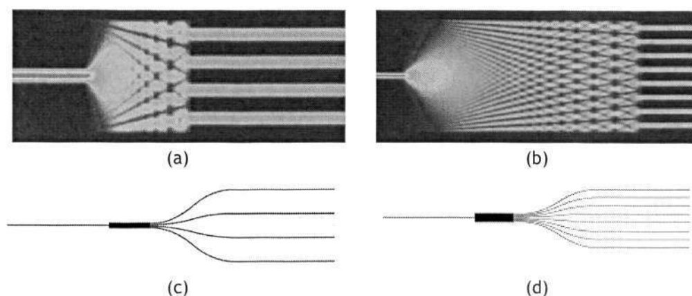
Fig.3.1.2. Simulation of designed (a) 1x4 and (b) 1x8 MMI power splitter and (c) 1x4 and (d) 1x8 MMI device with S-bend extensions used in fabrication.
