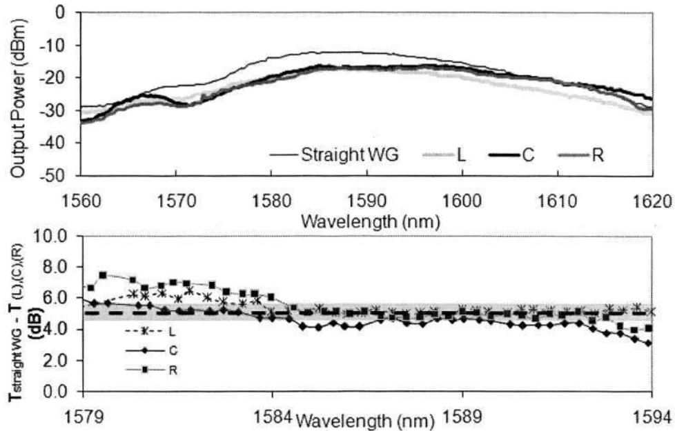
Fig. 3.5.4 (a) The measured output power of a straight waveguide, Output arms L, C and R (not normalized), (b) Insertion loss, or normalized output arm results of L(left arm), C(center arm) and R (right arm) obtained by obtaining the difference between the output from the straight waveguide and the different output arms.
