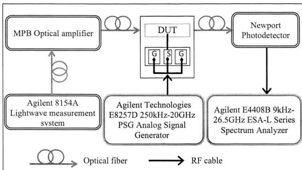
Figure 5.4.6 Schematic diagram of RF measurement setup for measuring EAM
