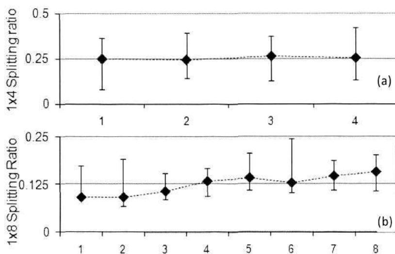
Fig.3.5.7. Splitting ratios and error bars for each output arms in the fabricated (a) 1\times 4 and (b) 1\times 8 MMIs.
