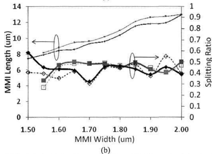
Fig. 4.2.7. (a)The left simulation illustrates a Type I MMI and the right simulation is a Type I* MMI. Both MMIs are 1.90\mu\text{m} wide. The Type I* MMI has a port pitch of 1.05\mu\text{m} . (b) Simulated Type I and Type I* MMI for MMI width 1.50 to 2.00\mu\text{m} wide shows different MMI lengths and splitting ratios for both cases. Black color plot denotes Type I MMI and Gray color plot denotes Type I* MMI. Bold lines are for the bar coupler and detached lines are for the cross coupler.
