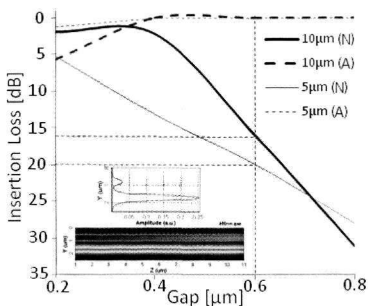
Fig. 4.2.3. Simulation of insertion loss vs. varying gap for 10 \mu\text{m} and 5 \mu\text{m} long parallel waveguides. (A) denotes the actual waveguide while (N) denotes the waveguide next to it. Inset shows the result of a 0.45 \mu\text{m} gap simulation.
