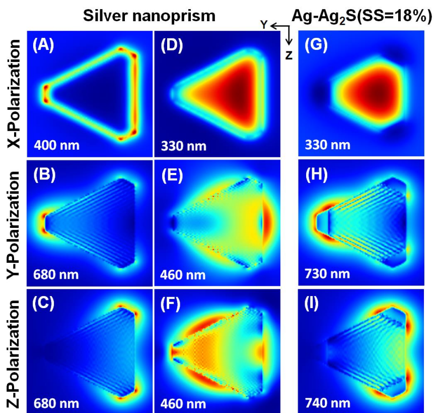
Figure 7. Near-field distribution calculated at different incident polarizations for (A-F) a pure silver nanoprism and (G-I) a Ag-Ag 2 S hybrid nanoprism with SS = 18\% . The near-field maps for the other SS values are reported in Figure S5-S9 in the Supporting Information.
