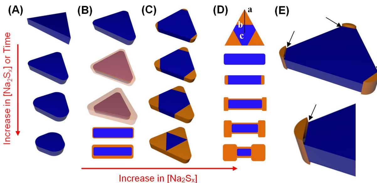
Scheme 1. (A-C) Proposed pathway of sulfidation processes as a function of \text{Na}_2\text{S}_x concentration: (A) C < 30 \mu\text{M} (B) 30 \mu\text{M} < C < 100 \mu\text{M} (C) C > 150 \mu\text{M} . (D) Nanoprisms' side view used to illustrate the change in height of hybrid nanoprisms for panel C. The top scheme defines the sulfidized section (SS) parameter, which is a radial ratio of \text{Ag}_2\text{S} and Ag from the tip of nanoprism to its center ( ab/ac ). (E) Diffusion sites of \text{S}_x^{2-} in the C > 150 \mu\text{M} range at the interface of Ag and \text{Ag}_2\text{S} are illustrated by the black arrows.
