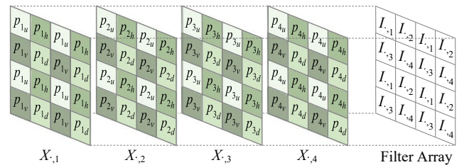
Fig. 7 The correspondence of pixel locations of sub-images, p_{ju} , p_{jh} , p_{jv} and p_{jd} , on X_{.j} , and input image channels, I_{.1} , I_{.2} , I_{.3} and I_{.4} , on polarization filter array, where the background colors of X correspond to those in Fig. 6.
