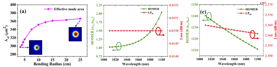
Fig. 3. (a) Calculated A_{eff} of LP 01 mode at 1065 nm in LMA-YDF-25/250-VIII fiber with different bending radii. (b) Calculated HOMER ( \alpha_{11}/\alpha_{01} ) (at left Y axis) and calculated loss of LP 01 mode (at right Y axis) in 12.5 cm radius bent LMA-YDF-25/250-VIII from 1010 nm to 1100 nm. (c) Calculated HOMER ( \alpha_{11}/\alpha_{01} ) (at left Y axis) and calculated propagation loss of LP 01 mode (at right Y axis) in designed AR-HCF from 1010 nm to 1100 nm.
