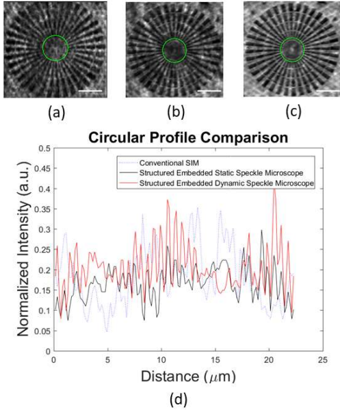
Fig. 10. Images obtained from the conventional SIM (a) is compared with structured embedded (b) static and (c) dynamic speckle illumination microscopy using Siemen's star as the test sample. The comparison of circular section profiles of the Siemen's star test chart indicated by the green circles in (a), (b) and (c) is shown in (d). The white scale bar in each image indicate 7.5 \mu\text{m} .
