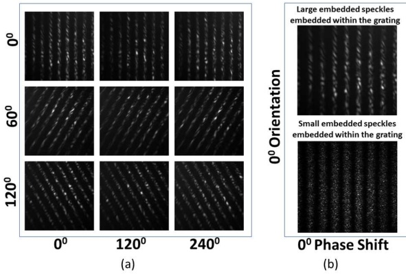
Fig. 3. (a) Modified SIM patterns incorporating speckle patterns, (b) different speckle sizes used for modulating the illumination grid having a 0°-orientation phase shifted by 0°. The speckle size variations are achieved by changing the size of the aperture placed after the diffuser.
