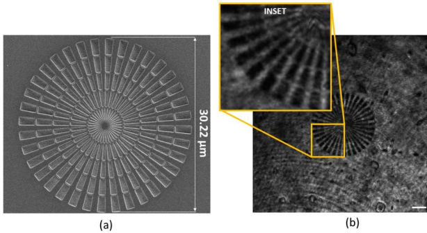
Fig. 6. Images obtained from a conventional SEM and a conventional microscope using a Siemen's star as the test sample. The white scale bar indicates 7.5 μm.
