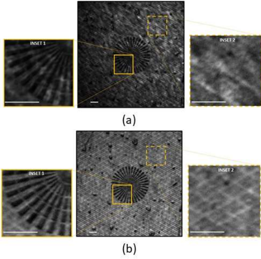
Fig. 9. Shows the images obtained from the structured embedded dynamic speckle illumination microscopy using a Siemen's star as the test sample with dynamic speckle patterns generated using (a) LSR-C-3005-1 and (b) LSR-C-3005-6D-VIS. Insets 1 and 2 represents the resolvable Siemen's star spokes and the reduced artefacts errors, respectively. The white scale bar in each image indicate 7.5 \mu\text{m} .
