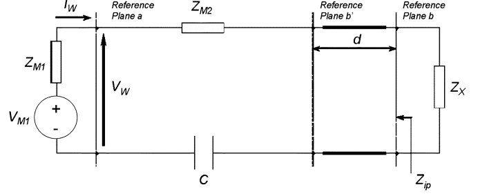
Fig. 6. Equivalent circuit for the two-current-probe setup.
