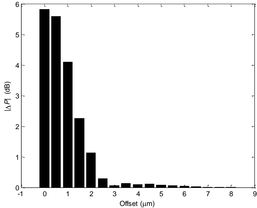
Figure 84: Transmission difference between refractive index 1.33 and 1.34 for offset 0 \mu\text{m} to 8 \mu\text{m} . The micro-channel dimension is 80 \times 4 .
