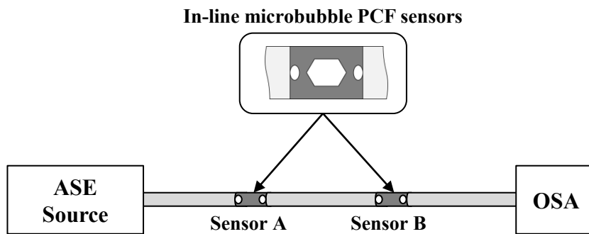
Figure 17: Experimental setup for the cascaded refractive index sensors.
