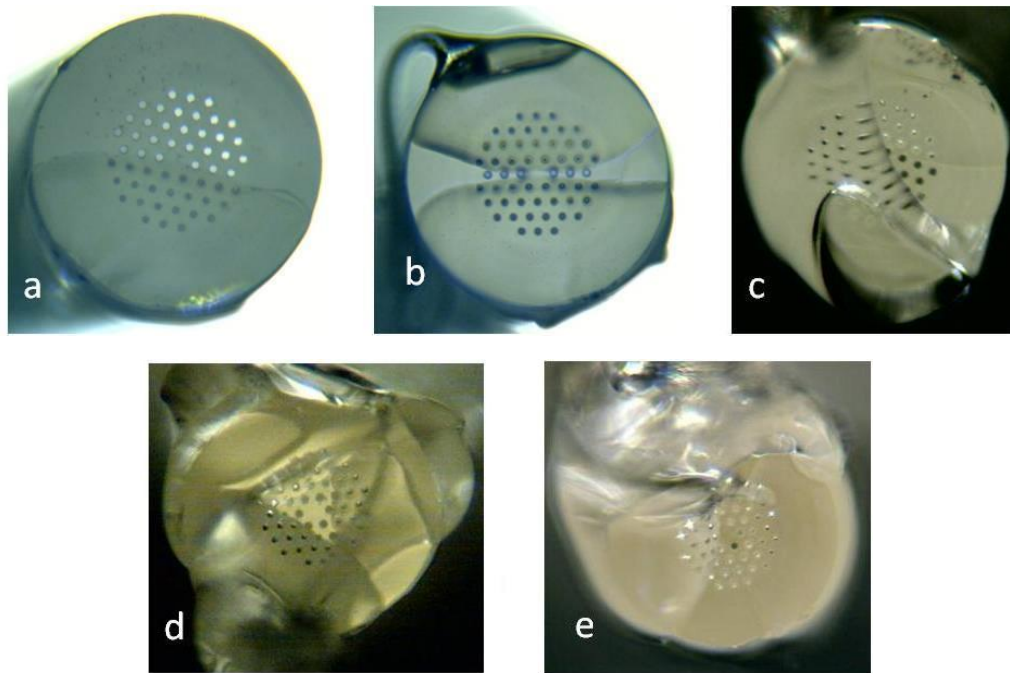
Figure 41: Microscope image of blocking patterns on the LMA-25 PCF. (a) About half of the air holes are unblocked; (b) center row of air holes are unblocked; (c) a pie-shaped of air holes are unblocked; (d) a triangle-shaped of air holes are unblocked; (e) a single air holes is unblocked and used for selective infiltration. Cladding diameter is 268 \mu\text{m} for reference.
