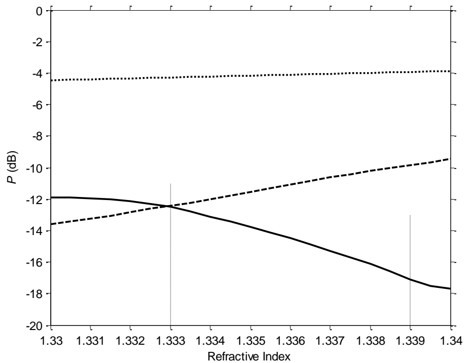
Figure 69: Calculated transmission power, P , for three different micro-channels' dimension as a function of refractive index. Solid line denotes 80 \times 4 .
