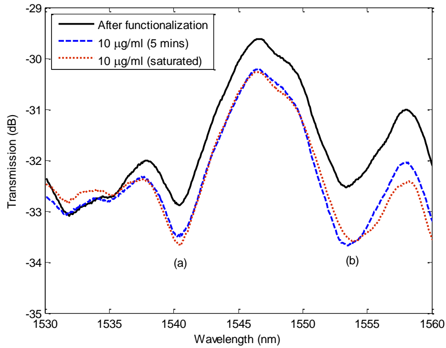
Figure 37: Measured spectrum of the biosensor during bioaffinity test. The streptavidin concentration is 10 µg/ml of PBS solution. Black solid line plots the spectrum after the functionalisation. Blue dashed line plots the spectrum after five minutes. Red dotted line plots the spectrum after streptavidin-biotin binding has saturated.
