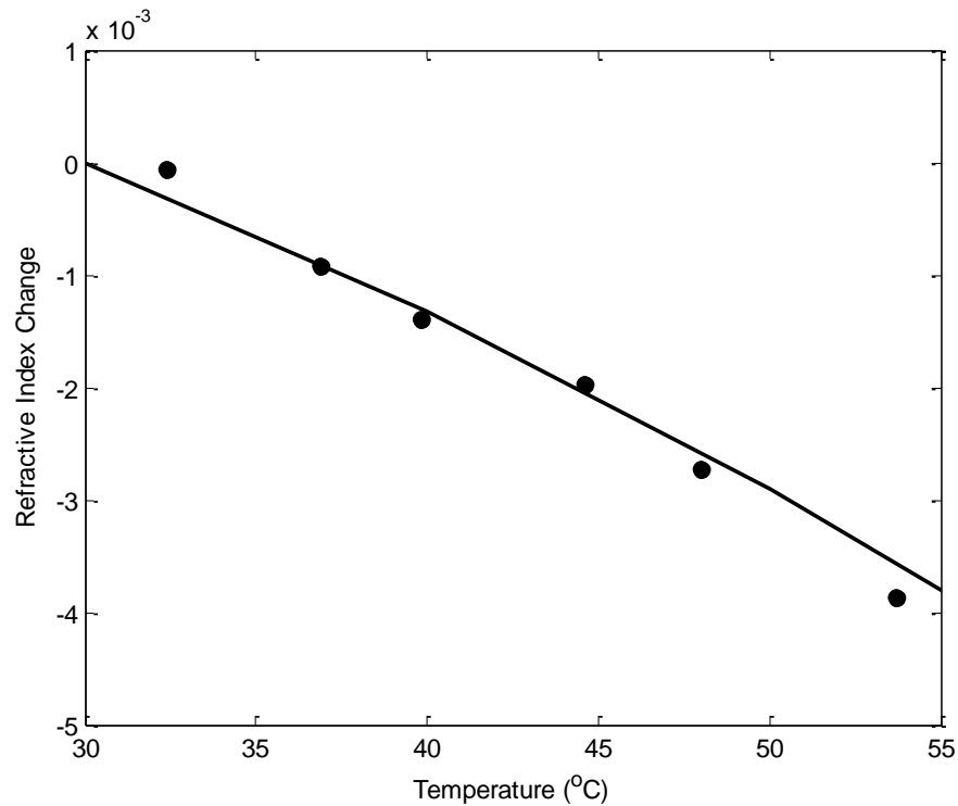
Figure 30: Calibrated refractive index as a function of temperature change.
