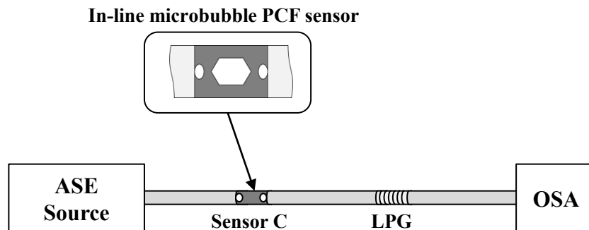
Figure 25: Experimental setup for the dual parameter sensor.
