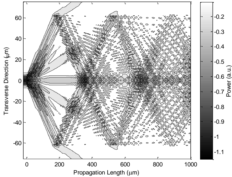
Figure 78: Beam propagation of 80×5 inside a single mode fiber.
