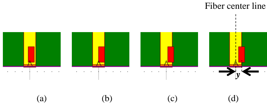
Figure 80: Micro-channel at (a) 10 μm, (b) 20 μm, (c) 30 μm, and (d) 40 μm offset from the center of the core.
