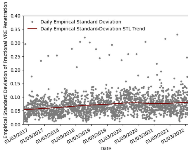
Fig. 11. Britain's standard deviation of fractional variable renewable energy penetration. Daily and trend.
