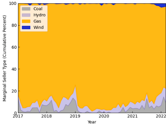
Fig. 14. Monthly Marginal Seller Type in the British Energy Imbalance Market (2017–2022). Ordered by average energy price (GBP/MWh) when each type is the marginal seller.
