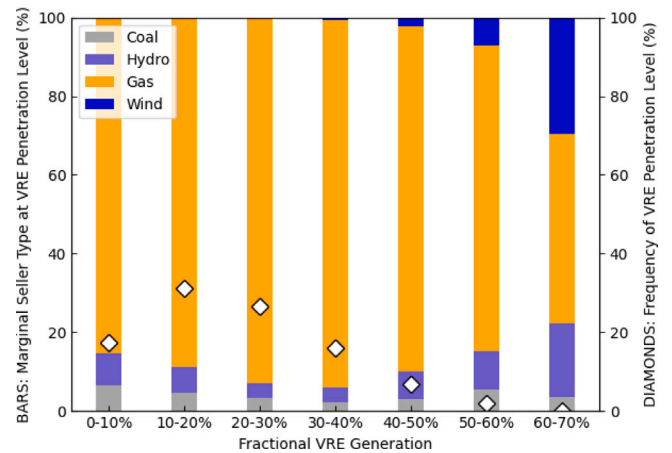
Fig. 15. Bars display the marginal seller generation type (as a percentage) during differing levels of VRE penetration. Diamond markers display the percentage of time periods during which this level of VRE penetration occurred. For example, while wind was the marginal seller 29.63% of the time when overall VRE penetration was at 60%–70%, VRE penetration rarely reached this level of contribution.
