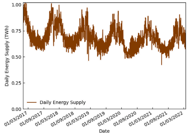
Fig. 8. Britain's daily energy (electricity) load (TWh).
