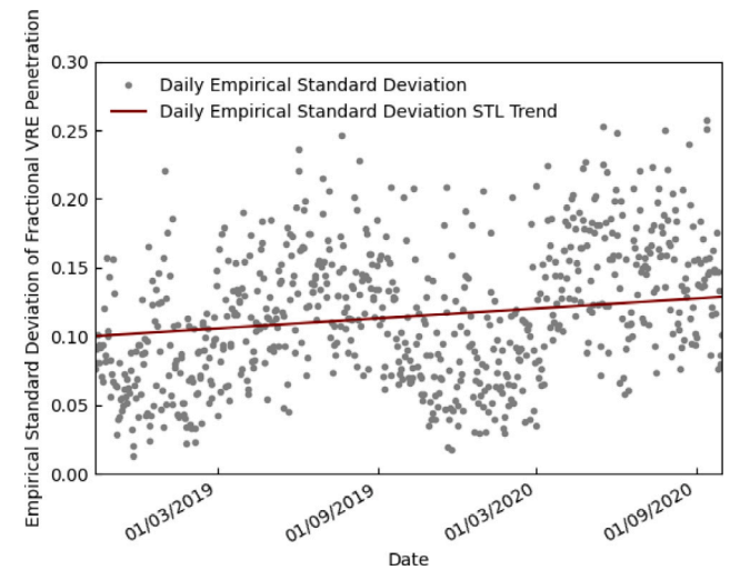
Fig. 5. Germany's standard deviation of fractional variable renewable energy penetration, and trend.
