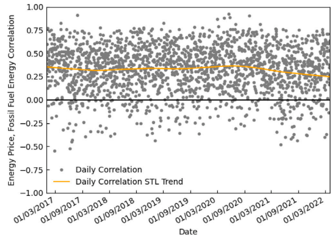
Fig. 10. Britain's energy price (GBP/MWh) to fractional fossil fuel energy penetration correlation.
