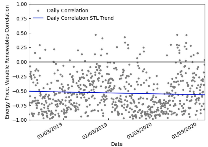
Fig. 4. Germany's energy price (EUR/MWh) to fractional variable renewable energy penetration correlation, and trend. This trend is persistently negative.
