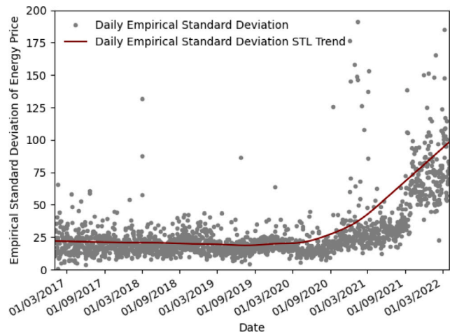
Fig. 12. Britain's standard deviation of the spot energy price and associated trend. Due to several outlier prices, this image is cropped for readability, with the full version shown in Figure A17 of the supplementary Material.
