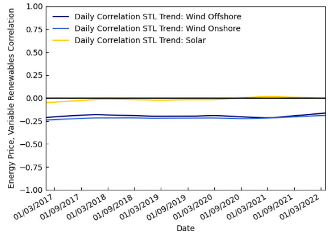
Fig. 13. Seasonal trends of Britain's energy price (GBP/MWh) to fractional offshore wind, onshore wind, and solar (PV) penetration correlation.
