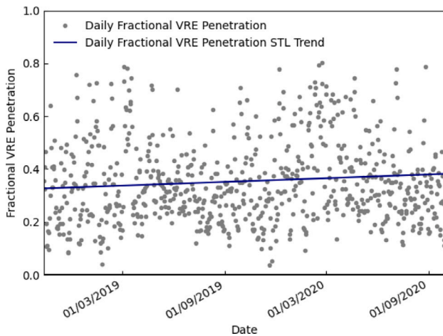
Fig. 1. Germany's fractional variable renewable energy (VRE) penetration (i.e. fractional generation) and seasonal trend of VRE penetration from 2019 to 2020. Points display the daily values, while the line shows the trend.
