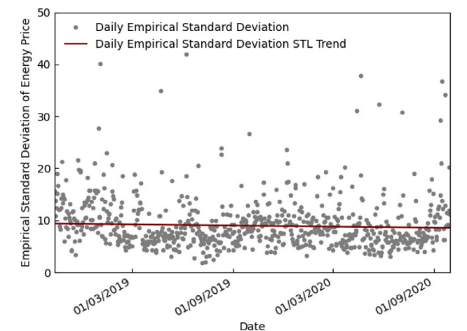
Fig. 6. Germany's standard deviation of energy price, and trend.
