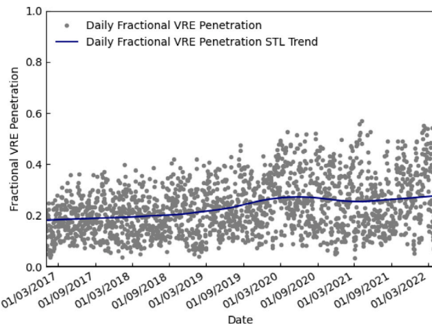
Fig. 2. Britain's fractional variable VRE penetration and seasonal trend of VRE penetration from 2017 to 2022. Points display the daily values, while the line shows the trend.
