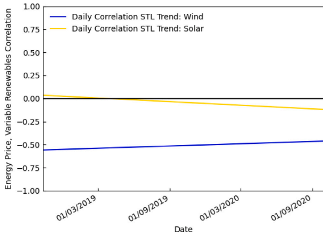
Fig. 7. Seasonal trends of Germany's energy price (EUR/MWh) to fractional wind, and solar (PV) penetration correlation.
