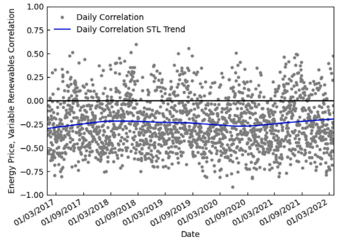
Fig. 9. Britain's energy price (GBP/MWh) to fractional variable renewable energy penetration correlation coefficient. The trend is persistently negative.
