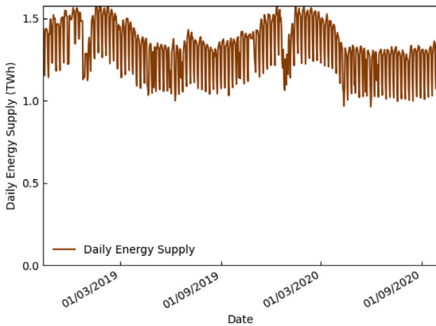
Fig. 3. Germany's daily electrical energy load (TWh).
