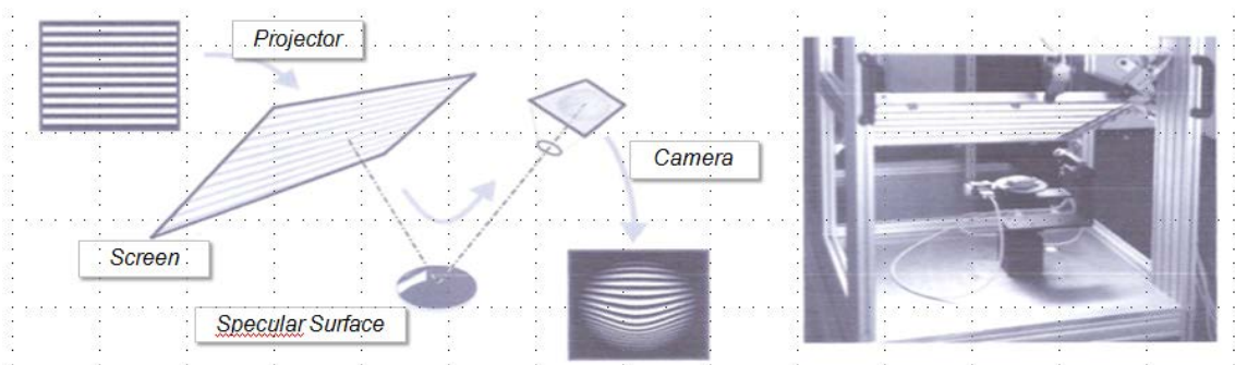
Figure 11: Experimentation set up of PMR
