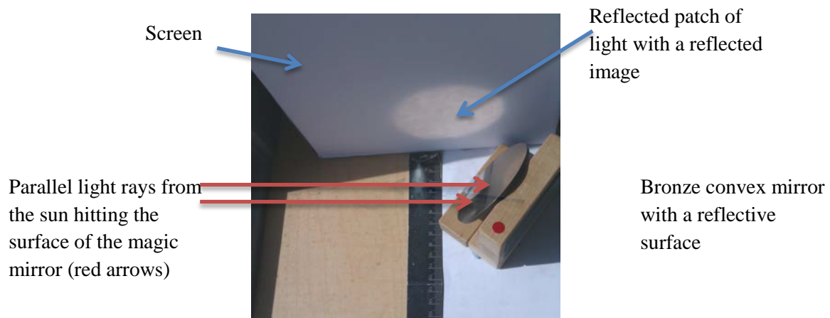
Figure 1: Magic Mirror principle
