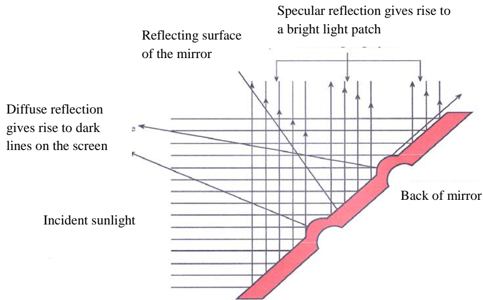
Figure 3: Dents cause reflections to go in different direction from the background.
