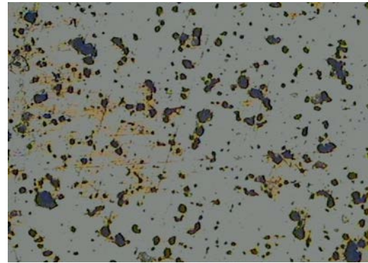
Figure 5: Surface of magic mirror observed with a magnification of (x10 / x15) under another optical microscope
