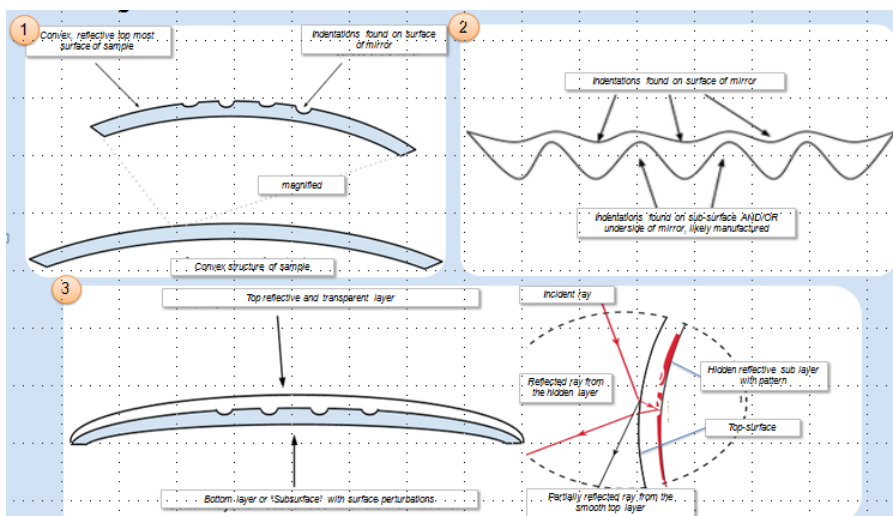
Figure 9: 3 distinct types of structures
