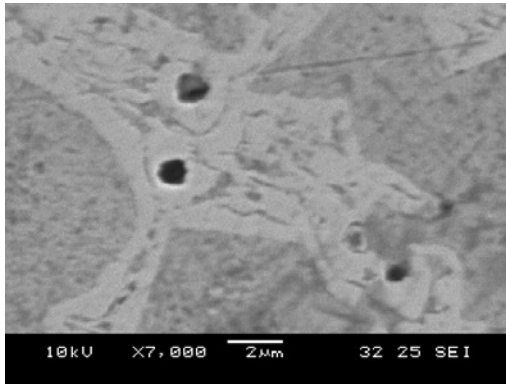
Figure 7: Results from the Scanning Electron Microscope
