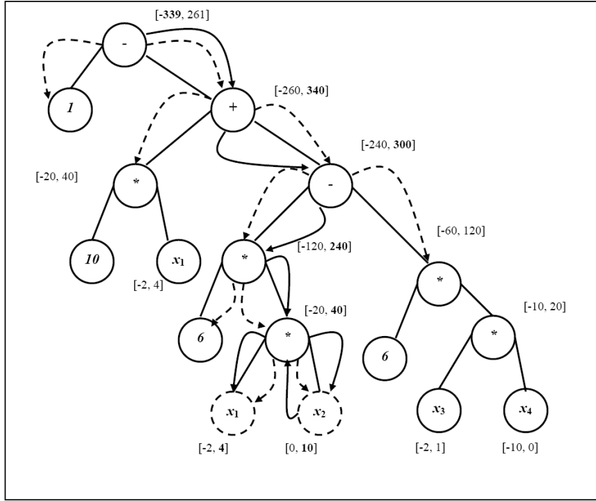
Figure 4.5. Implementation of IIR_Tree over the binary tree for “ 1-((10*x_1)+(6*(x_1*x_2)))-(6*(x_3*x_4))=0 ”
