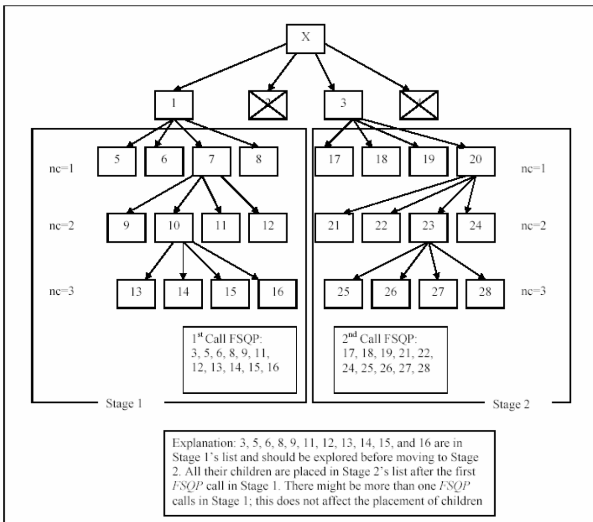
Figure 3.5. Implementation of the adaptive iterative deepening procedure.
