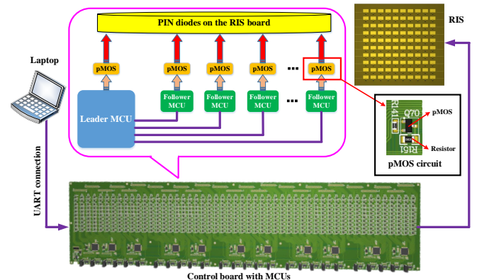
FIGURE 3. Demonstrating the connection relationship and signal transmitting progress of the whole RIS system with control circuitry.
