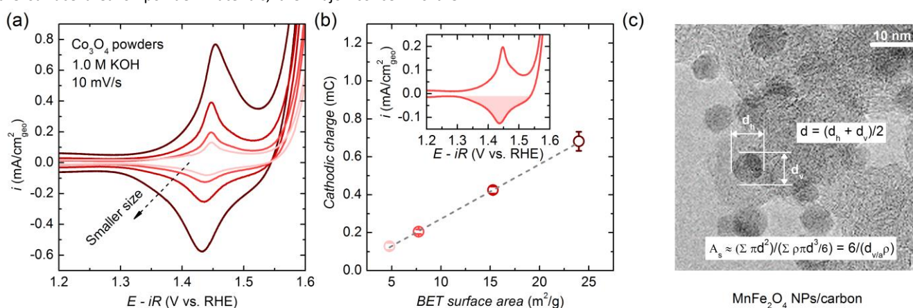
Fig. 7 (a and b) The correlation between the coulombic charge (Q) of surface redox reaction and Brunauer-Emmett-Teller (BET) surface area, which is exemplified by Co 3 O 4 spinel oxides 40 with various particles sizes. (a) CV of Co 3 O 4 (b) Q of cathodic Co 3+ /Co 4+ peak at various Co 3 O 4 as a function of BET surface area. Inset is an exemplary integration of cathodic Co 3+ /Co 4+ peak. (a and b) are reproduced from ref. 40 with permission from Elsevier, copyright 2018. (c) Determining the surface area ( A_s ) of MnFe 2 O 4 nanoparticles (NPs) 41 by transmission electron microscopy (TEM) image, where the measurement of particle size and calculation of A_s is shown. The NPs are loaded on Vulcan carbon. Reproduced from ref. 41 with permission from Springer Nature, copyright 2017.
